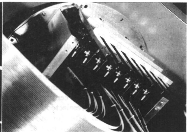
FIGURE 3.2-3. Detector Hybrid
