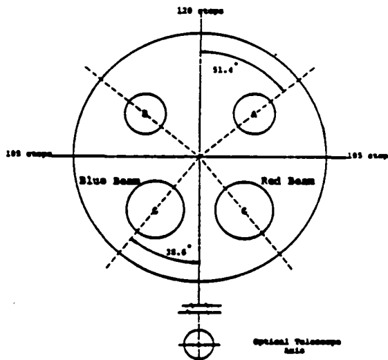
Figure 3. Relative configuration of the optical elements as viewed from inside the FOS in the direction of the entrance ports.
