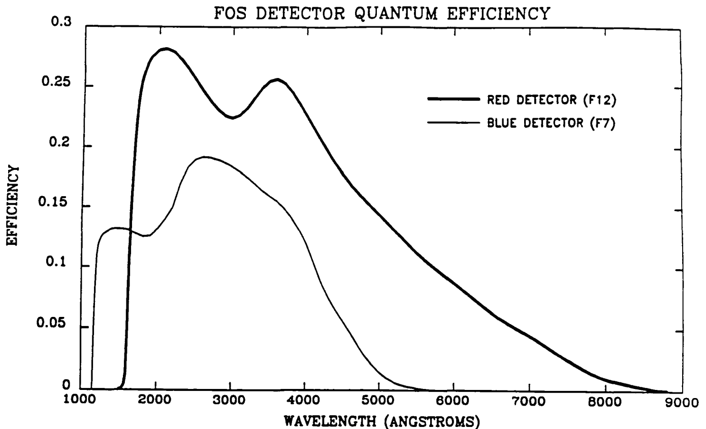
Figure 2.2.4-1 (revised) Quantum efficiency of the FOS Flight detectors.
