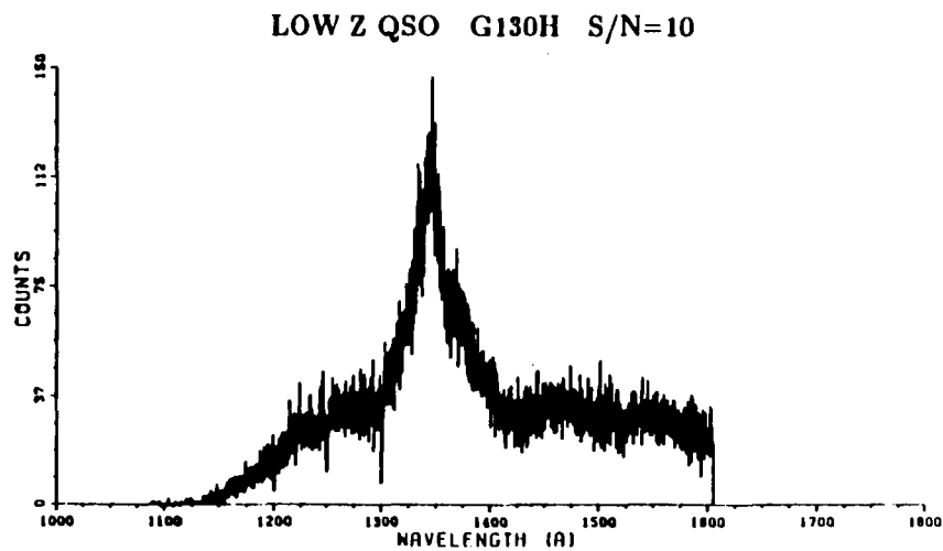
Fig. 4.1-2 Simulated FOS spectra of a low redshift quasar taken with grating G130H and the blue digicon. The signal-to-noise ratio (SNR) at a given wavelength is closely approximated by the square root of the number of counts per pixel at that wavelength. The strong emission feature is \text{Ly}\alpha , and the four absorption lines from blue to red have equivalent widths of 1 \text{ \AA} , 1 \text{ \AA} (a doublet consisting of two 0.5 \text{ \AA} lines separated by 1 \text{ \AA} ), 0.25 \text{ \AA} , and 1 \text{ \AA} .
