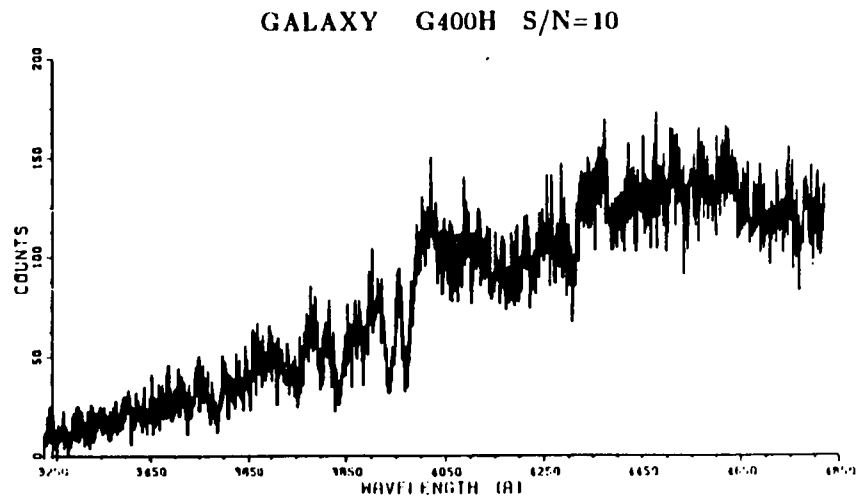
Fig. 4.1-8 Simulated FOS spectra of an early-type galaxy taken with grating G400H and the red digicon. Because the original data had a resolution of 10 \text{ \AA} , which is less than grating G400H's 3 \text{ \AA} resolution, the spectra approximate observations of a galaxy which has a velocity dispersion of several hundred \text{km sec}^{-1} .
