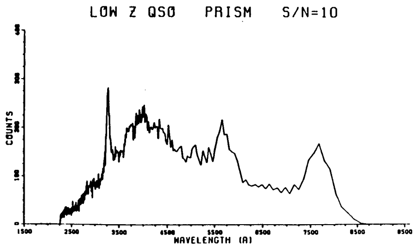
Fig. 4.1-1 Simulated FOS spectra of a low redshift quasar taken with the prism and the red digicon. The signal-to-noise ratio (SNR) is given at the central pixel, which corresponds to a wavelength of approximately 3250 Å. The nonlinear spectrum has been rebinned to a linear scale. The three sharp peaks correspond to MgII 2800, H \beta , and H \alpha at a redshift of 0.17.
