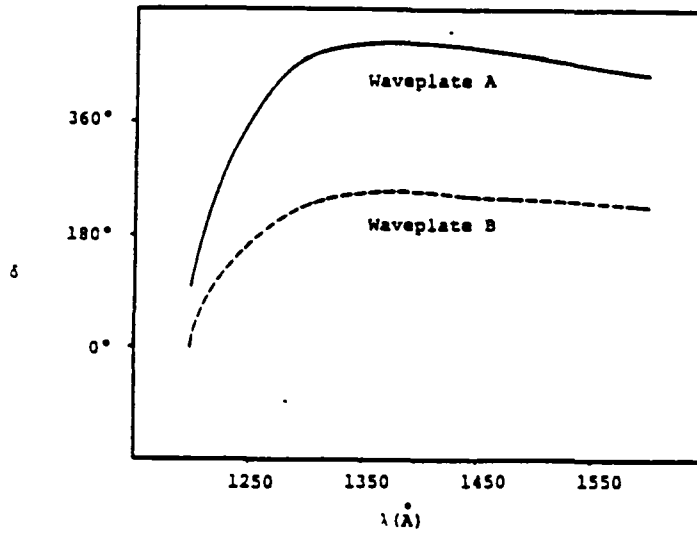
Figure 4. Retardations of the flight waveplates.
