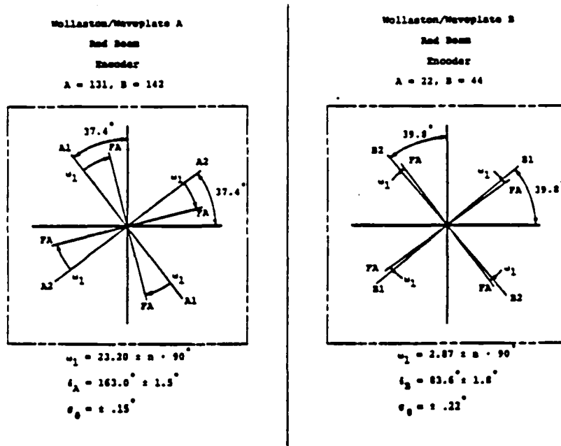
Figure 7. Diagrams of the Wollaston pass directions and the initial positions of the waveplates that were derived from the operational tests of the polarimeter.
