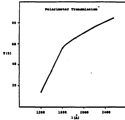
Figure 5. The transmission of the polarimeter as a function of wavelength.
