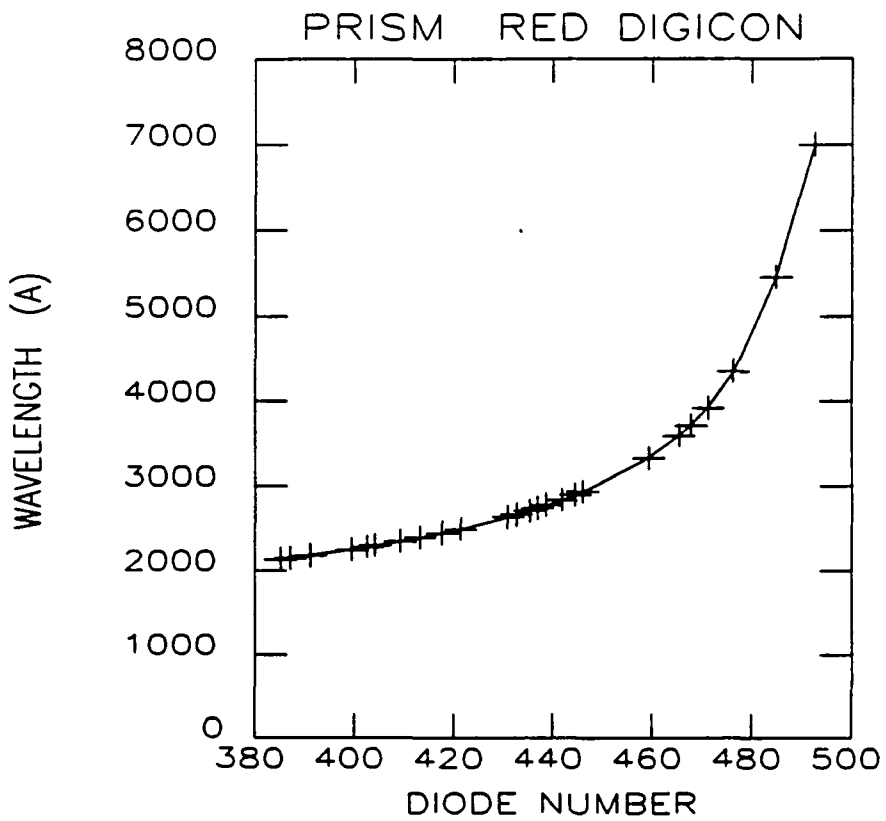
Figure 2.2.3-1. Wavelength as a function of pixel number for the prism with the blue and red Digicon (Sirk and Bohlin 1985).
