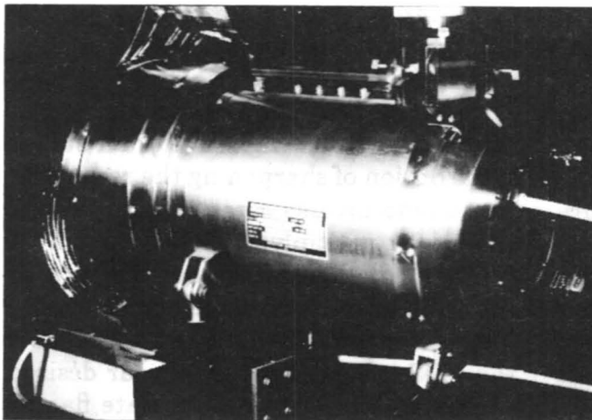
FIGURE 3.2-2. Red Flight Detector. Preamplifiers. The 512 preamps fit into back end of detector assembly. Each set consumes less than 10 watts.
