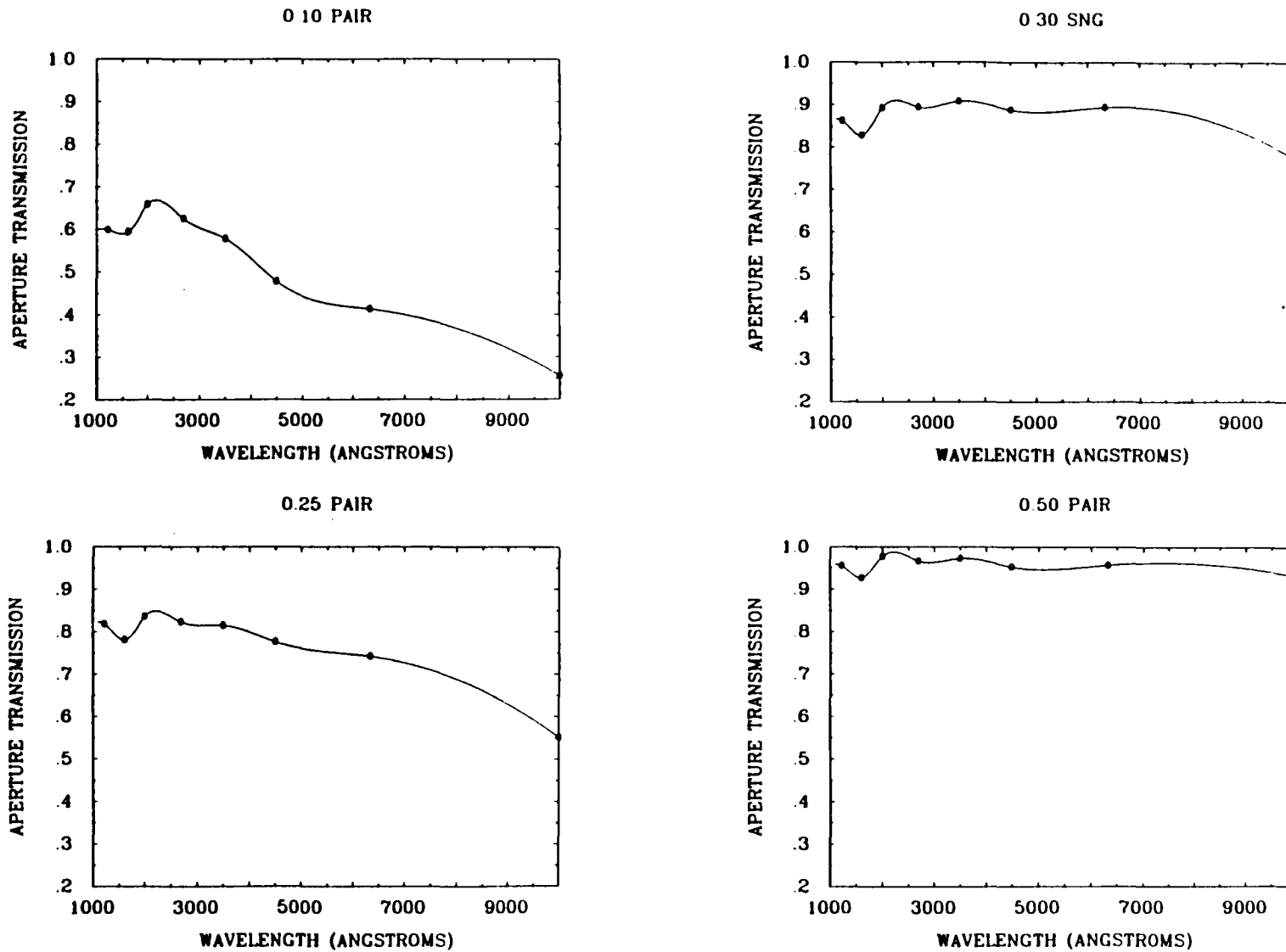
Fig. 4.2-2 Fraction of light transmitted by the apertures for a perfectly centered point source. The curves for the 0.10 PAIR and the 0.25 PAIR include the fraction of light lost from the aperture diffraction pattern which overfills the FOS collimator.
