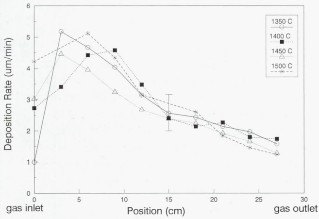
Figure 1.—Deposition rate vs. position for Group A.
