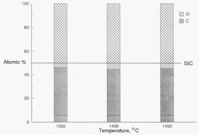
Figure 4.—Electron microprobe analysis of CVD SiC (Group B).
