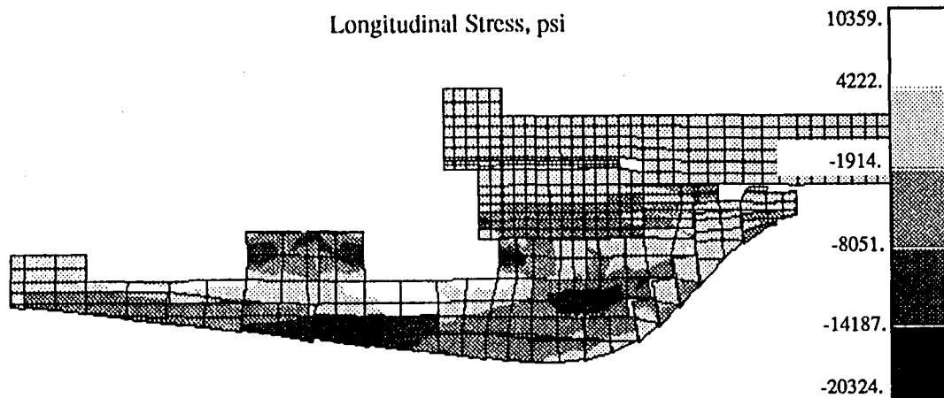
Figure 3. Stress / Deformation Plot under Preload w/gaps = .026/.018
