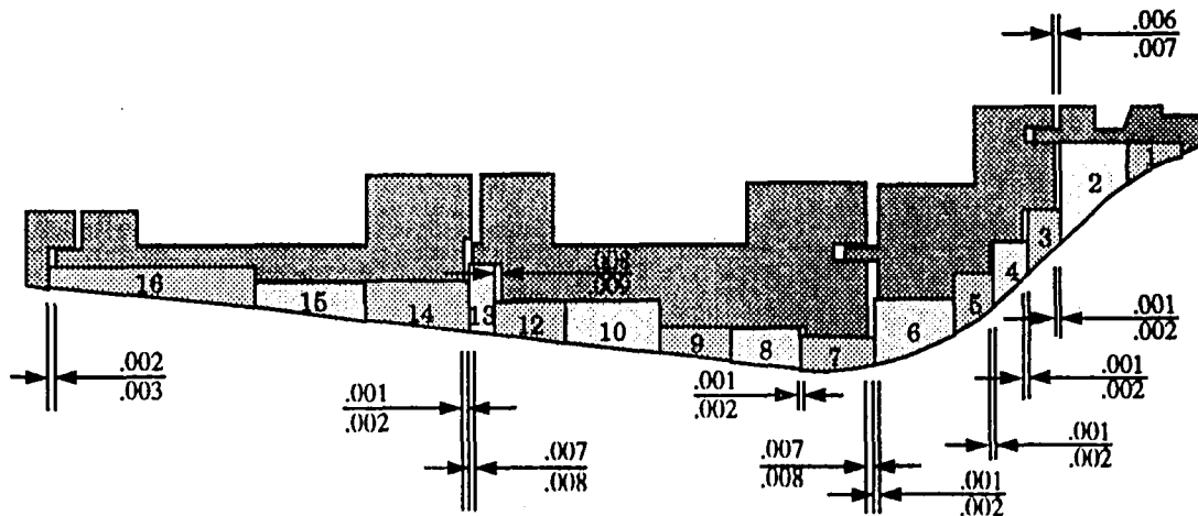
Figure 7. Tolerance Layout.
