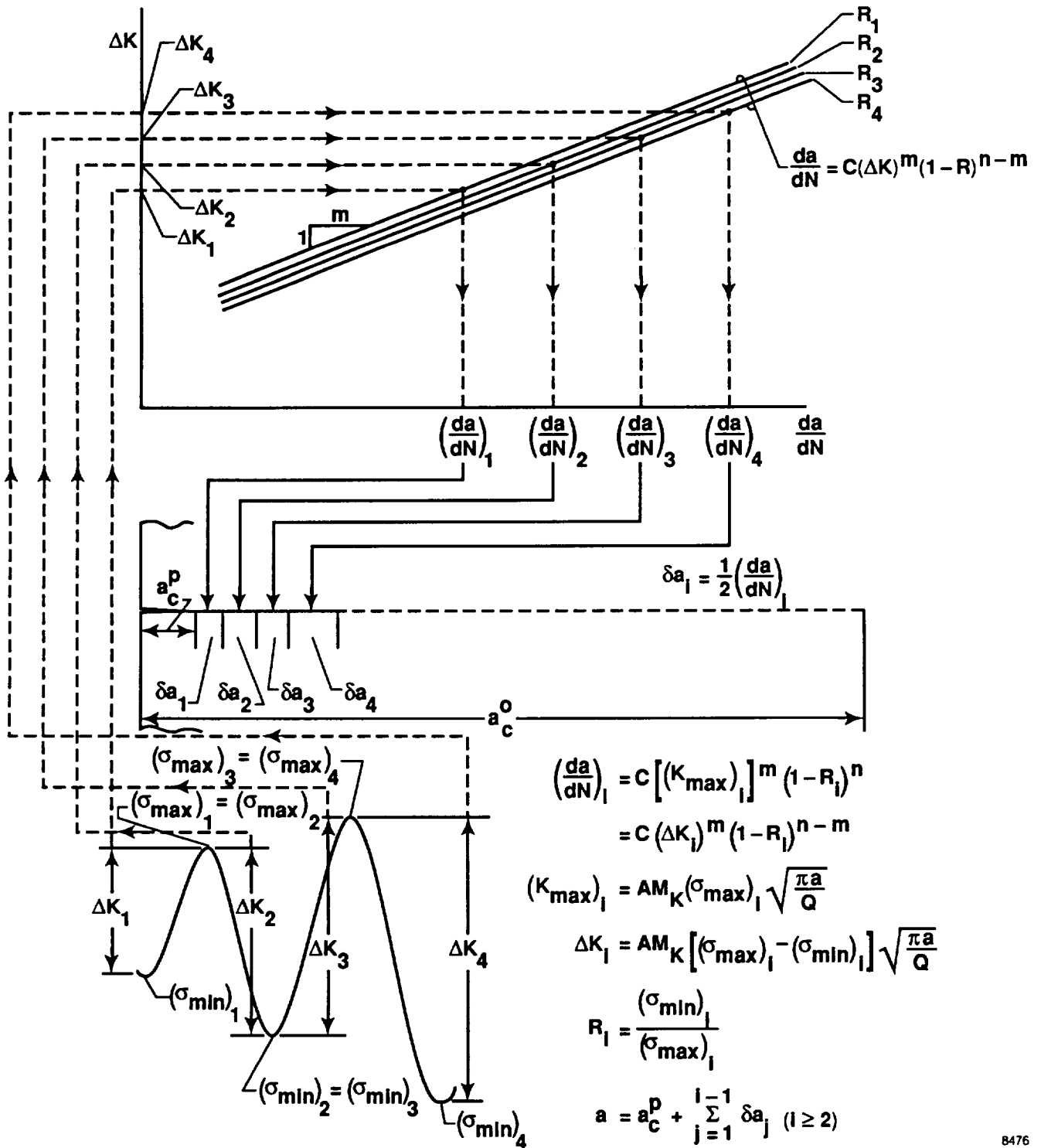
Figure 3. Graphic evaluation of crack increments for random stress cycles using half-cycle method.
