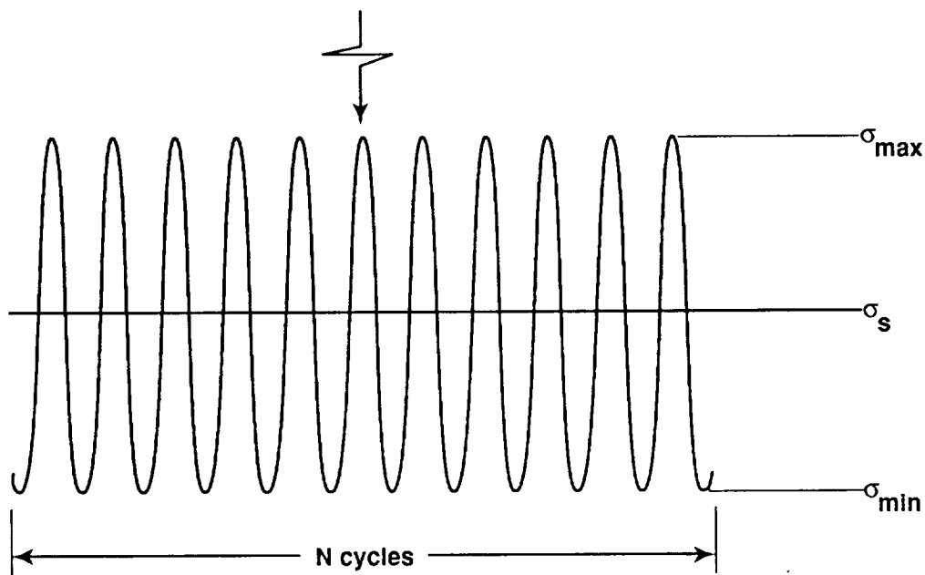
(b) Constant-amplitude stress cycles.
