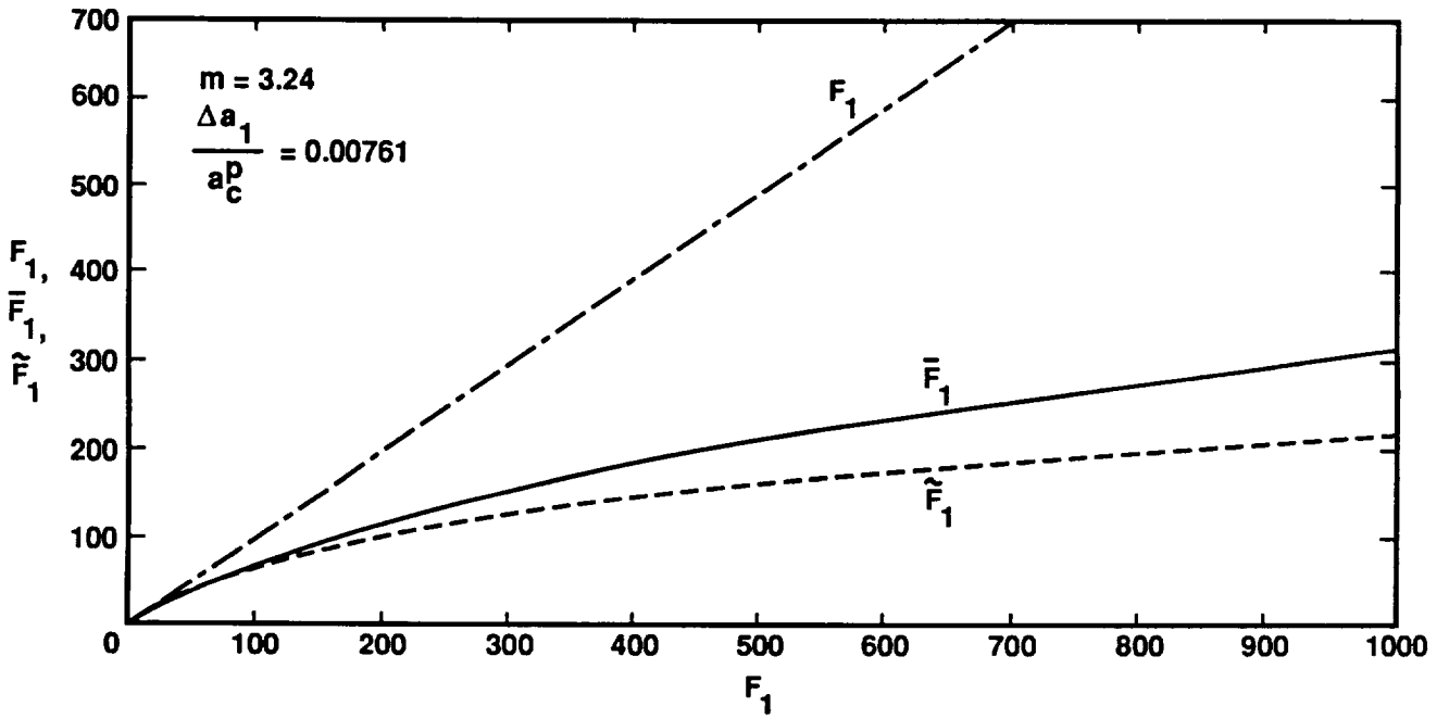
Figure 9. Comparison of number of remaining flights predicted from conventional theory and the first- and second-order theories; rear hook.
