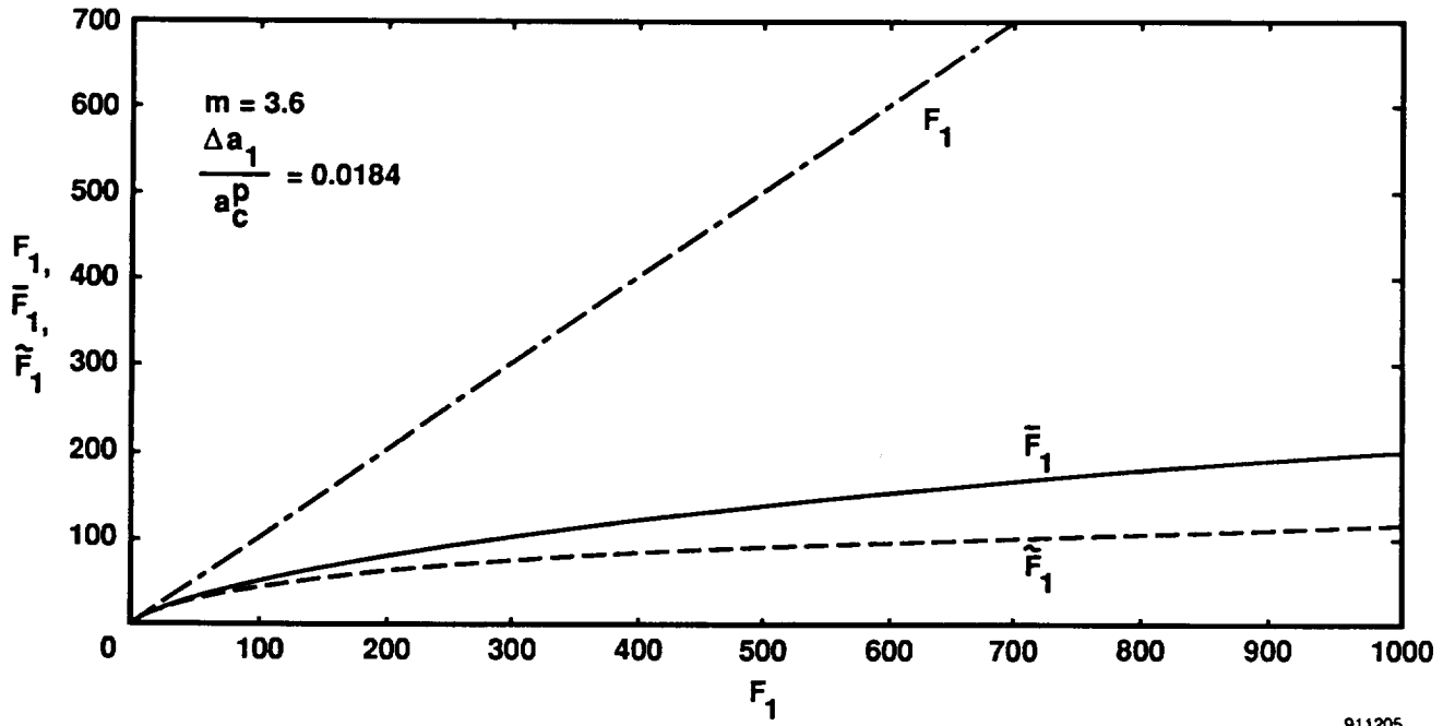
Figure 8. Comparison of number of remaining flights predicted from conventional theory and the first- and second-order theories; front hook.
