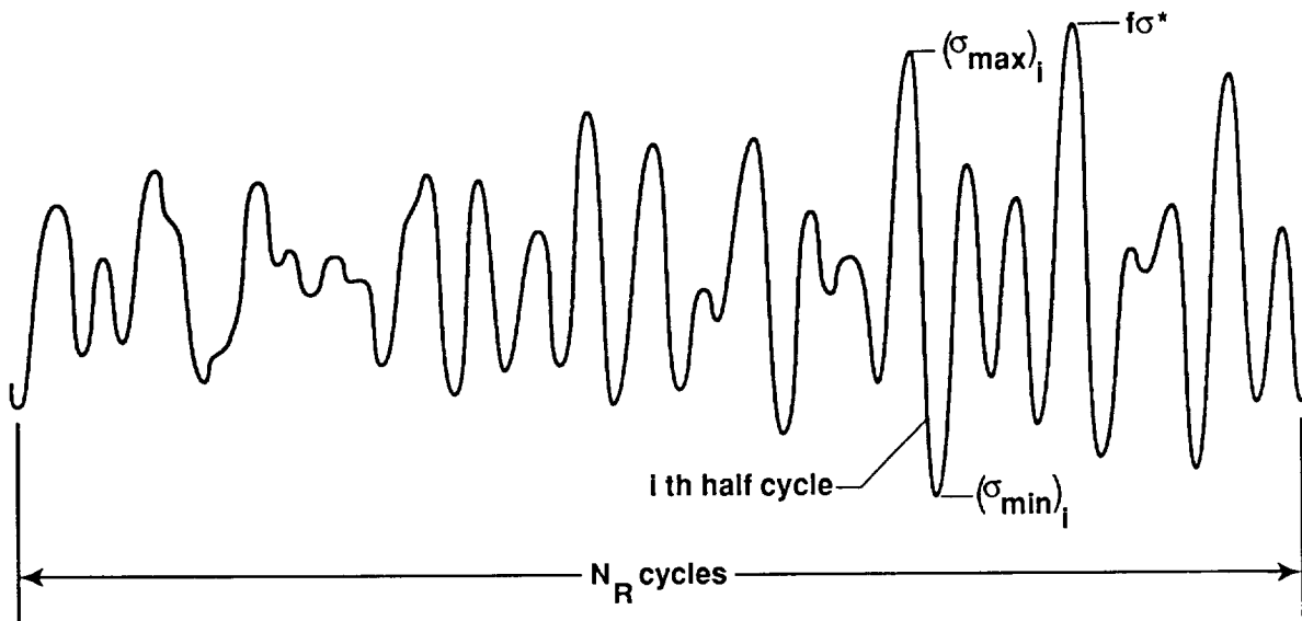
(a) Random stress cycles.
