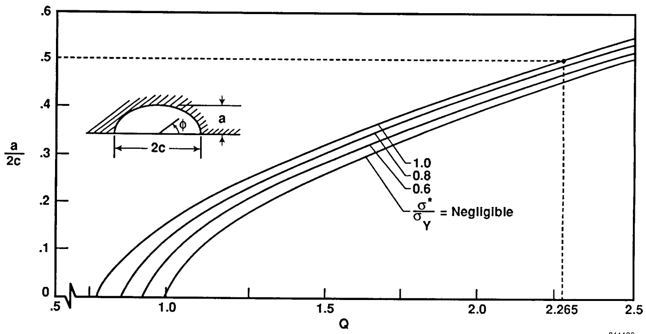
Figure 1. Surface flaw shape and plasticity factor for semielliptic surface crack.
