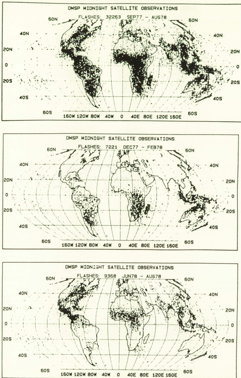
Fig. 4. Top , one year of DMSP-OLS midnight lightning discharges for 365 consecutive days for the period September 1977 to August 1978; Middle , DMSP-OLS midnight lightning for the N. hemisphere winter December 1977 to February 1978; Bottom , DMSP-OLS midnight lightning for the N. hemisphere summer June-August 1978 (after Orville and Henderson, 1986).
