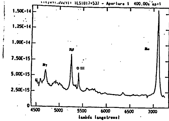
Figure 2: Redshifted MDM 1.3 m spectrum of the serendipitous Slew Survey AGN 1ES1817+537 ( z = 0.08 ). Exhibits Balmer emission ( H\alpha , H\beta , H\gamma ) and weaker O III \lambda\lambda 4959, 5007 .
