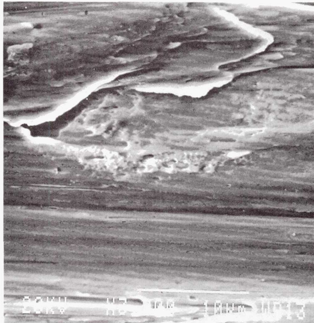
Figure 25.—SEM photomicrograph of wear track showing extensive plastic shearing in Inconel 718 disk after sliding against dry-film-lubricated Ti-6Al-4V pin in air then rerun in vacuum.
