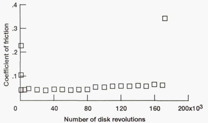
Figure 12.—Coefficients of friction for dry-film-lubricated Ti-6Al-4V pin sliding against Inconel 718 disk at 8.5 N in vacuum.
