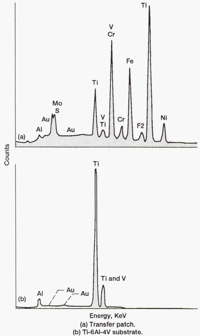
Figure 22.—EDX analysis of wear scar produced in dry-film-lubricated Ti-6Al-4V pin after sliding against Inconel 718 disk in air and then rerun in vacuum. The thin gold film used to reduce charging of the mount is responsible for the gold signal in the two spectra.
