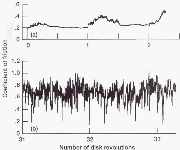
(a) At first and second revolution. (b) At 31st and 32nd revolution.
