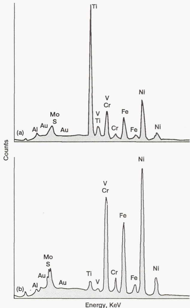
(a) Transfer patch of Ti-6Al-4V. (b) Smear area.
