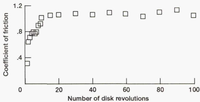
Figure 11.—Coefficients of friction (highest value) for unlubricated Ti-6Al-4V pin sliding against Inconel 718 disk as function of number of disk revolutions at 4 N in vacuum.
