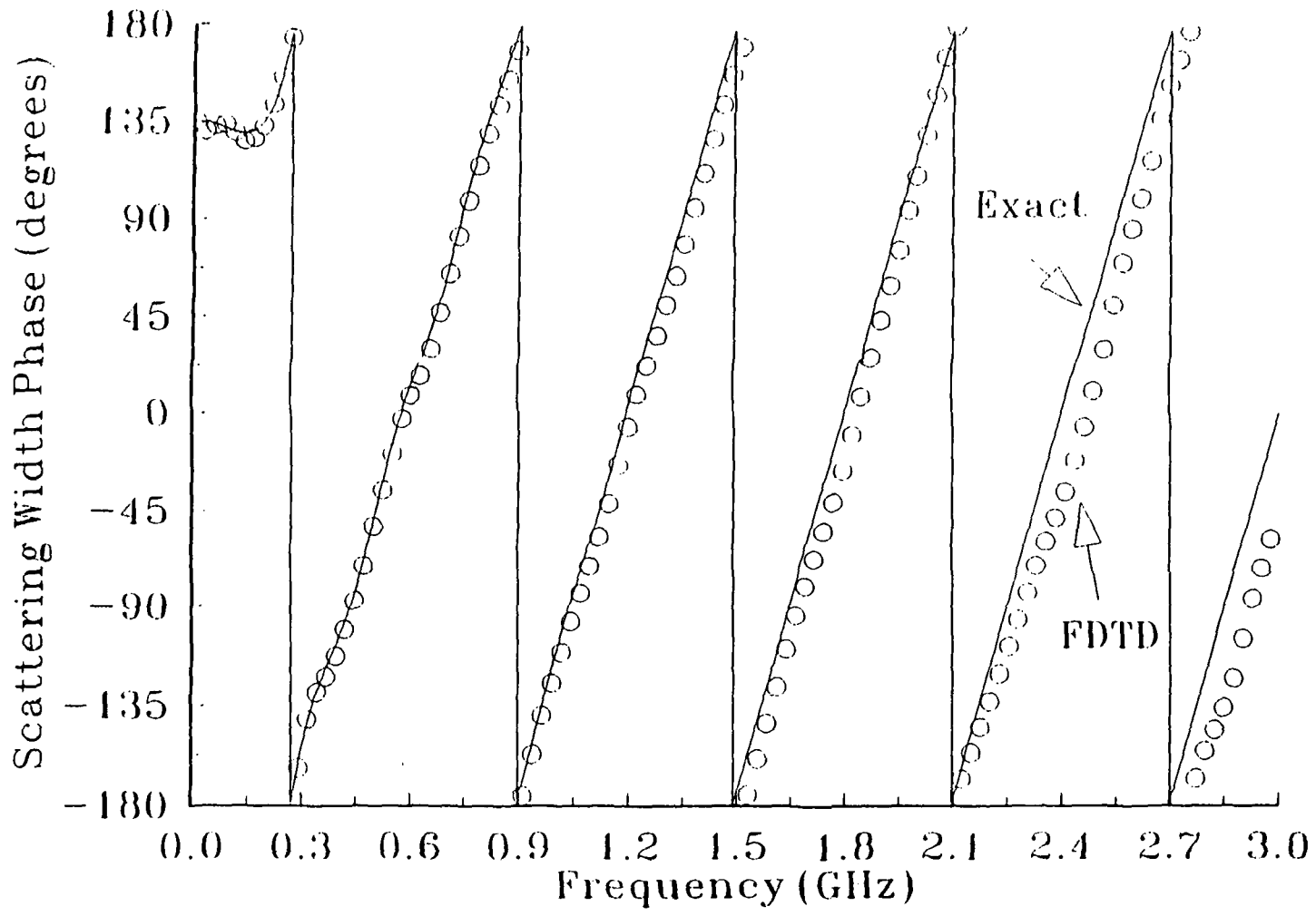
PEC Cylinder, TE z , 200x200 FDTD space Radius 0.25 meters
