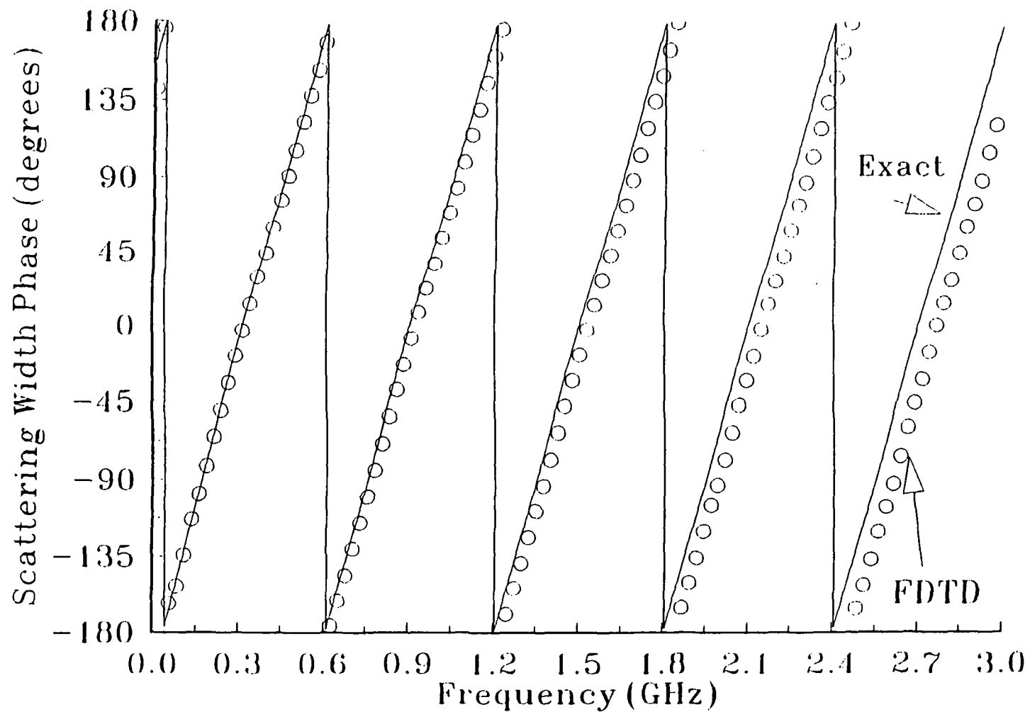
PEC Cylinder, TM_z , 500x500 FDTD space Radius 0.25 meters
