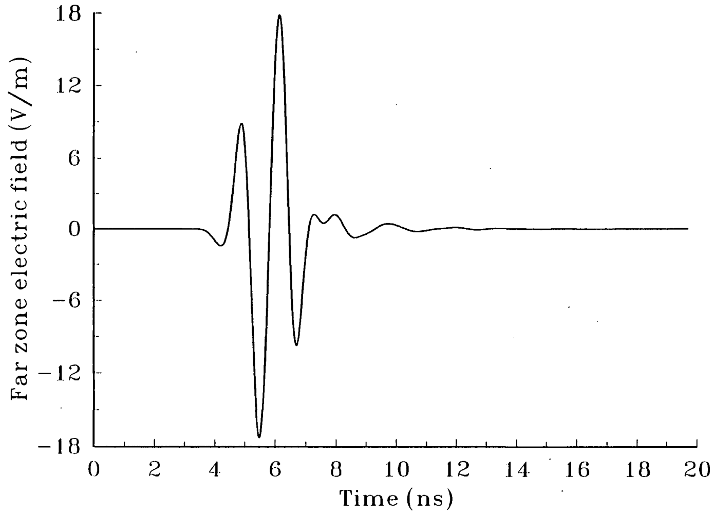
Cross-polarized far zone scattered field 29 cm square PEC plate; \vartheta=45 , \varphi=30 degrees
