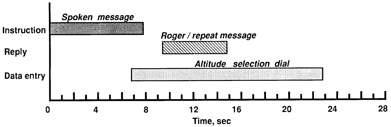
(a) Conventional voice radio.
