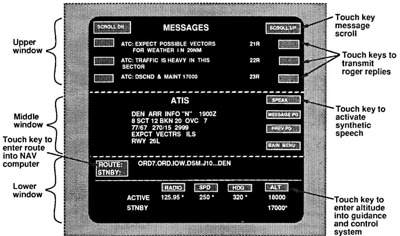
Figure 4. Display format of three-window data link interface.
