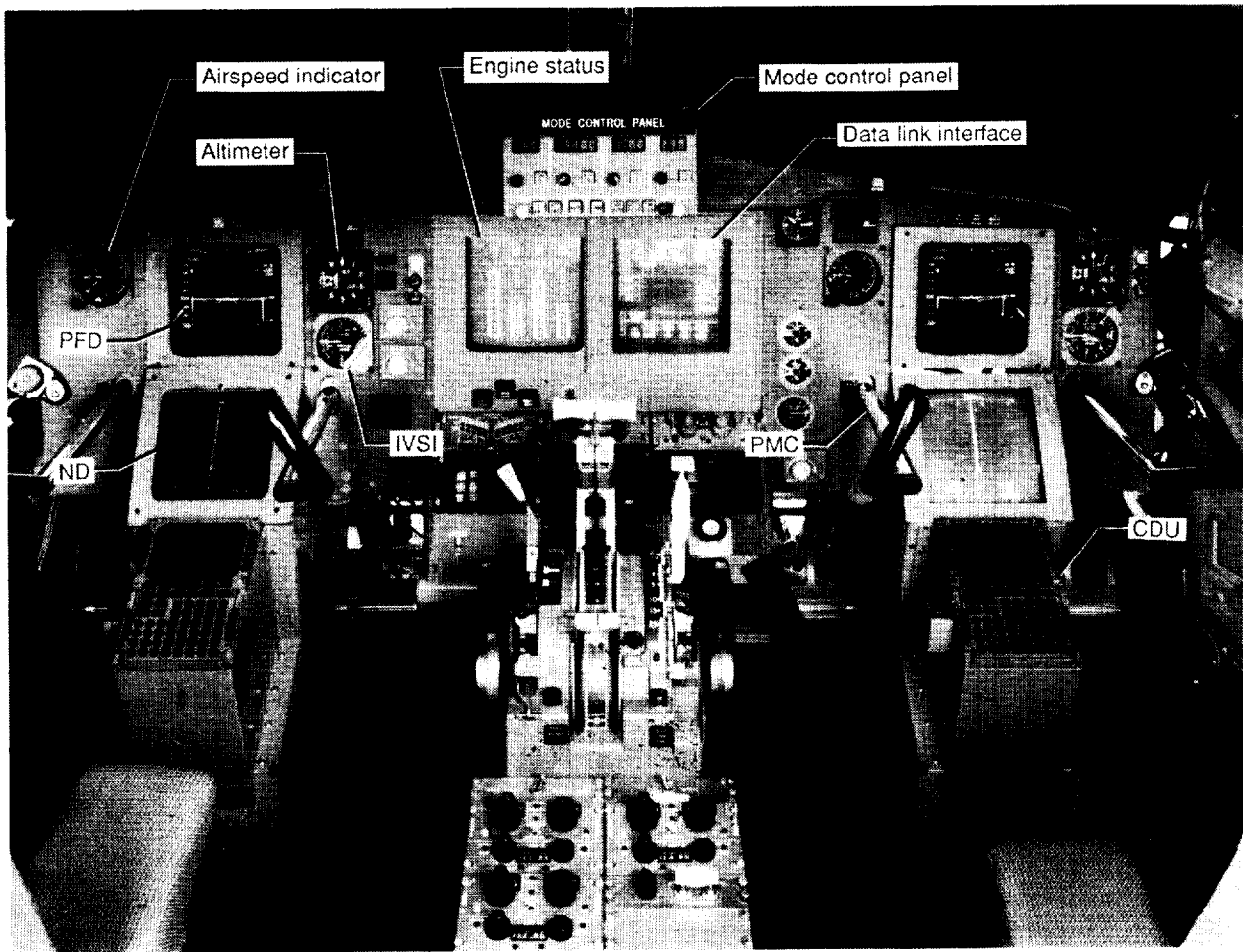
Figure 1. Transport Systems Research Vehicle Simulator.
