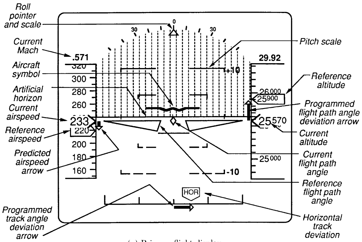
(a) Primary flight display.
