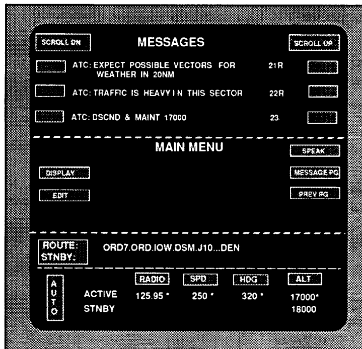
Figure 20. Altitude clearance data swapped to active area.
