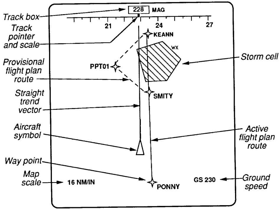
(b) Navigation display (ND).
