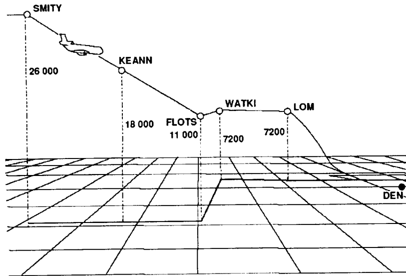
(c) Nominal descent and approach path. (Altitudes are in feet.)
