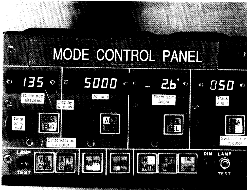
Figure 3. Mode control panel.
