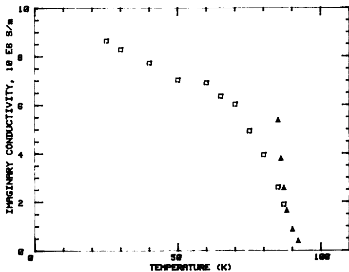
FIGURE 4. Imaginary part of the conductivity, \sigma_2 , versus temperature for 0.7 \mu\text{m} (□) and 0.4 \mu\text{m} (Δ) laser ablated \text{YBa}_2\text{Cu}_3\text{O}_{7-\delta} thin films on \text{LaAlO}_3 at 35 GHz.
