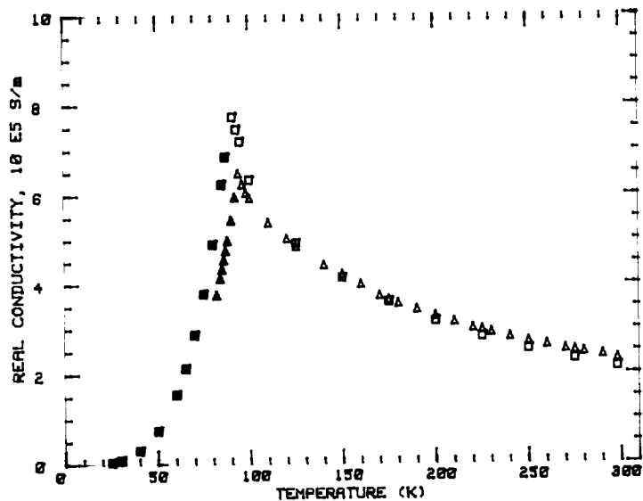
FIGURE 3. Real part of the conductivity, \sigma_1 , versus temperature for 0.7 \mu\text{m} (□) and 0.4 \mu\text{m} (Δ) laser ablated \text{YBa}_2\text{Cu}_3\text{O}_{7-\delta} thin films on \text{LaAlO}_3 at 35 GHz; \sigma_1 = \sigma_N for T > T_c and \sigma_1 = \sigma_1 for T < T_c . Open symbols represent values of the conductivity calculated directly from power transmission measurements and filled symbols represent values of the conductivity calculated using the two-fluid model.
