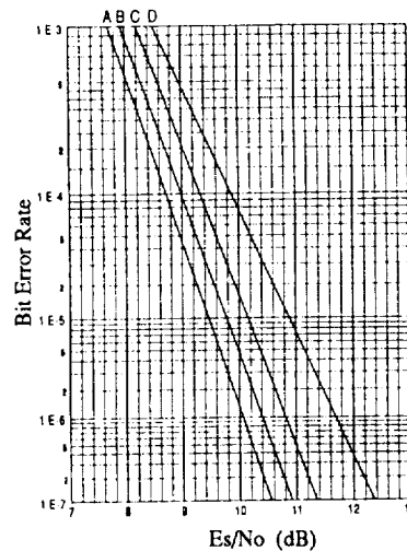
CODED 4x4 QAM COMPUTER SIMULATION RESULTS
