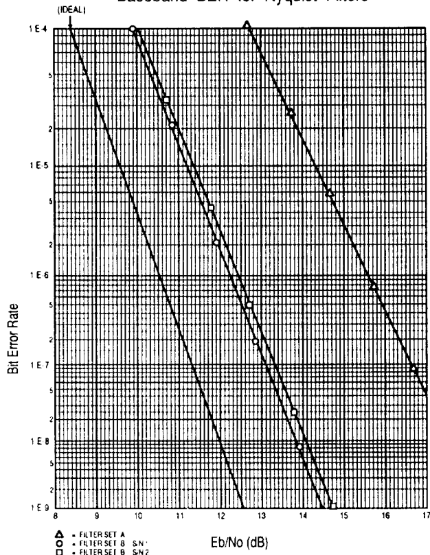
Baseband BER for Nyquist Filters
