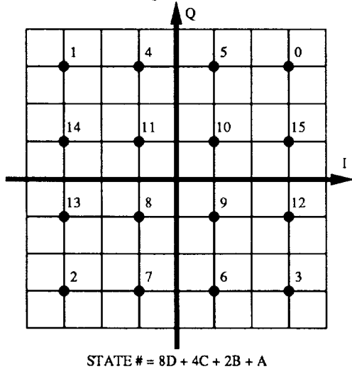
IDEAL 4X4 QAM PHASE PLANE
