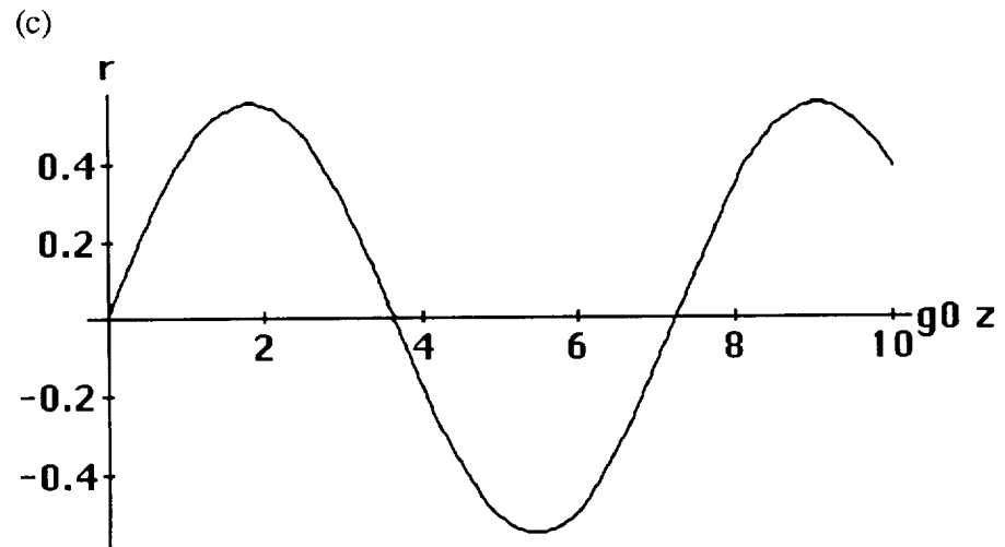
Fig 1. Squeezing magnitude as a function of propagation distance z measured in gain lengths g_0 , for different values of phase mismatch \Delta k : (a) \Delta k = 0.1g_0 , (b) \Delta k = g_0 , (c) \Delta k = 2g_0 .
