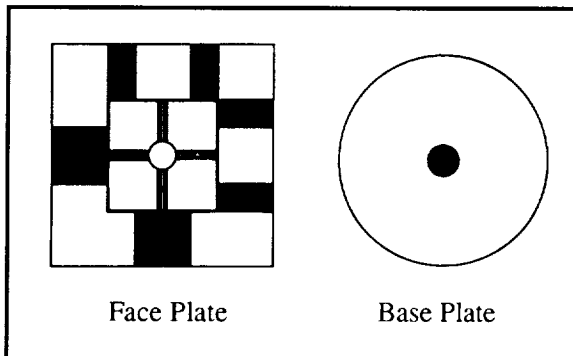
Figure 1. Face plate and base plate concepts incorporated into the original Spar target.
