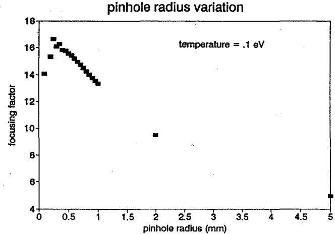
Figure 6.—Effect of pinhole size on focus factor.
