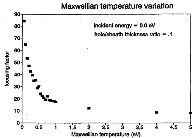
Figure 7b.—Effect of temperature on focus factor for an incident energy of 0.0 eV.
