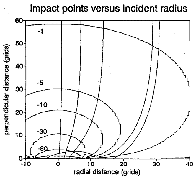
Figure 4.—Examples of particle trajectories.
