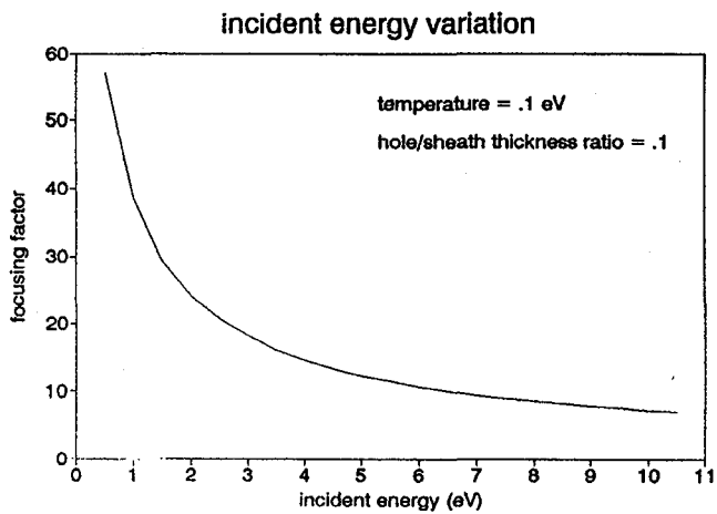
Figure 5.—Relationship between energy of incident particles and resulting focus factor.
