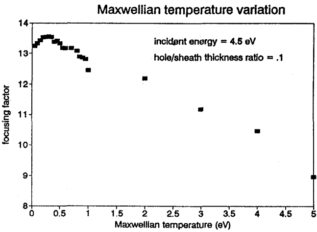
Figure 7a.—Effect of temperature on focus factor for an incident energy of 4.5 eV.
