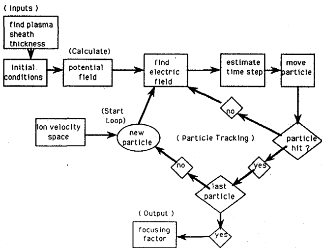
Figure 3.—Schematic diagram of program flow.
