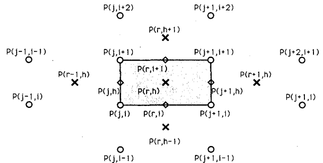
Figure 2.—Potential interpolation scheme.
