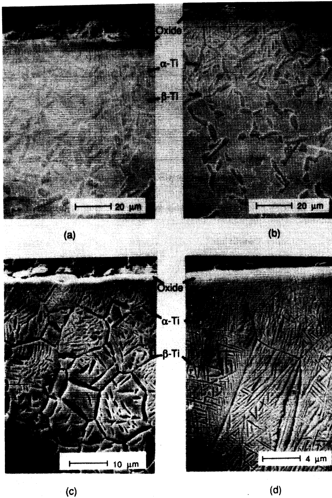
Figure 3 - SEM Micrographs of Beta-21S Exposed at (a) 800°C for 30 hr, (b) 800°C for 100 hr, (c) 700°C for 72 hr, and (d) 600°C for 72.5 hr.
