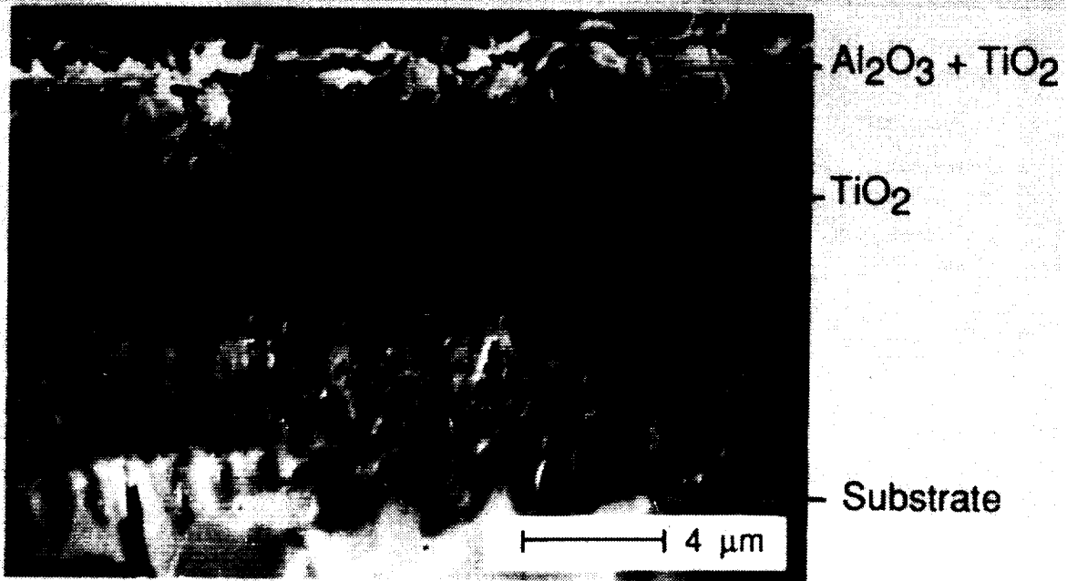
Figure 2 -SEM Micrograph of Beta-21S Exposed at 800°C for 100 hr
