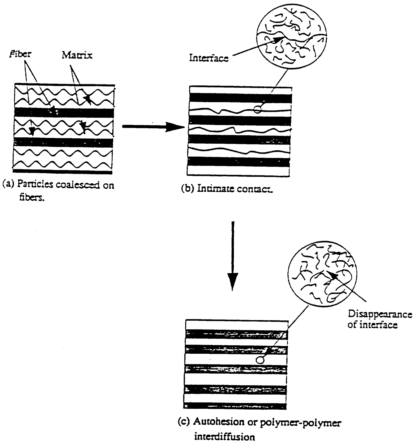
Consolidation of powder-impregnated thermoplastic composite.
