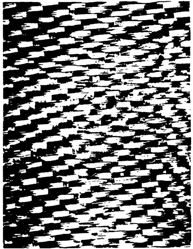
Figure 1a. Photograph of eight-harness satin cloth woven from no twist, 6k carbon fiber yarns prepregged with LARCR™-TP1 powder.
