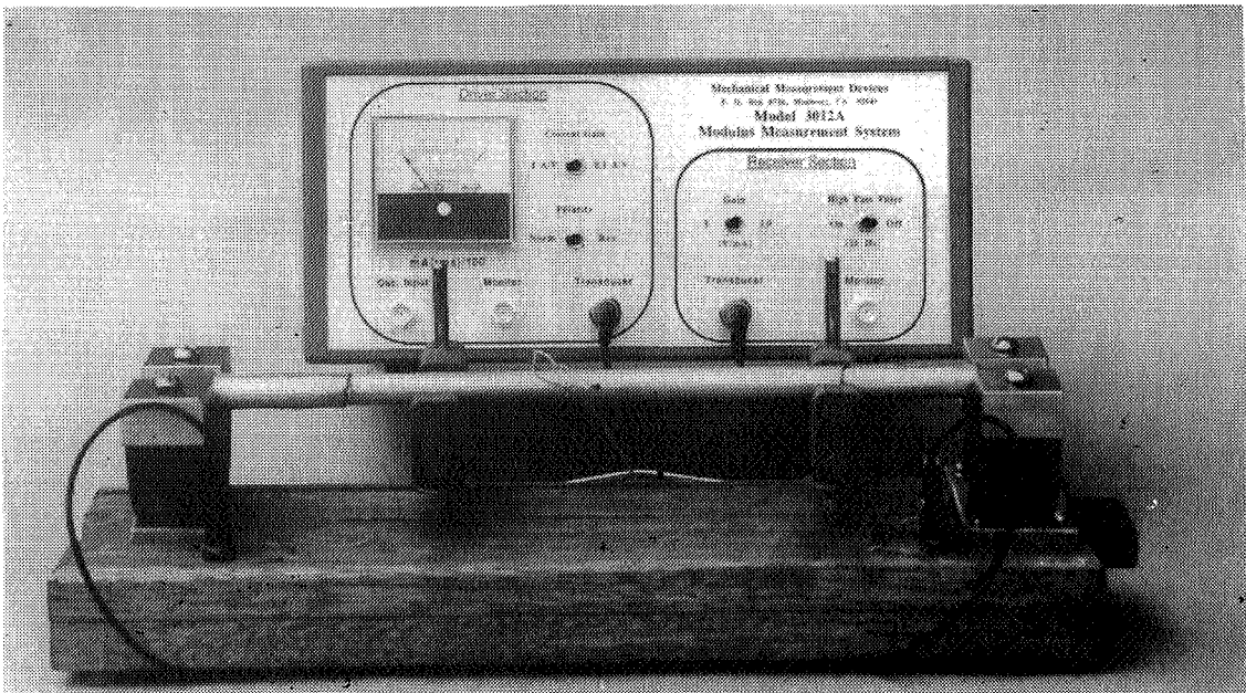
Figure 1. A measurement apparatus [11] used to electro-dynamically excite and detect the flexural, longitudinal, and torsional modes of a free-free bar for determination of the shear and Young's elastic moduli.
