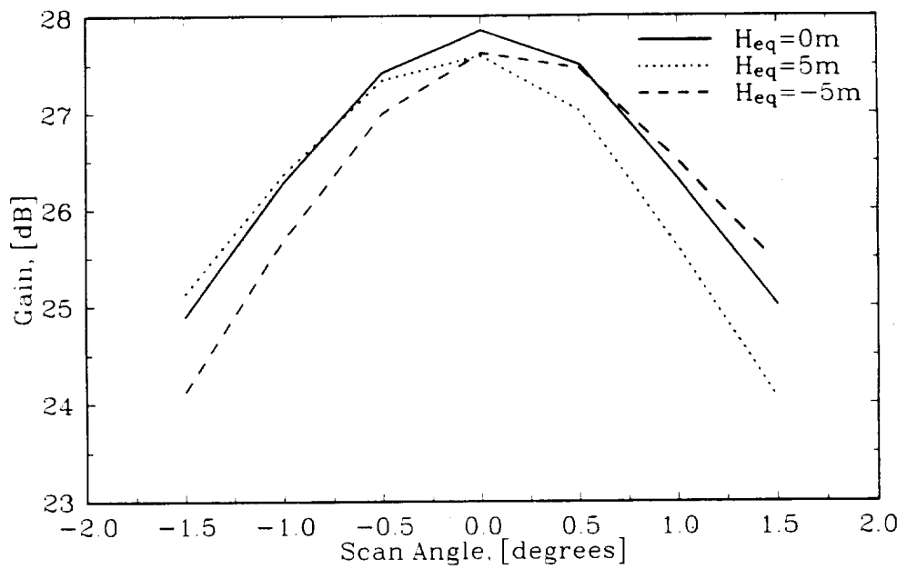
LaRC Test Article, Type 6, 10 GHz Scan by Feed Displacement
