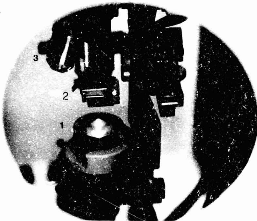
Figure 3. The ESA Biorack light microscope (breadboard) to be used in two Biorack experiments. Description starting below: (1) condensor, (2) sample holder with inserted culture chamber, (3) objectives, (4) beam splitter, (5) video camera, (6) eyepiece, (7) photo-diode assembly
