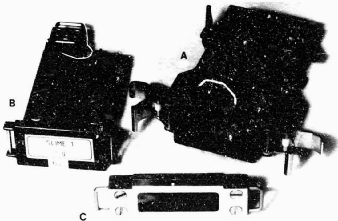
Figure 2. Hardware for the experiment (already used in D1): (A) Type I container, (B) holder for two culture chambers, and (C) culture chamber.
