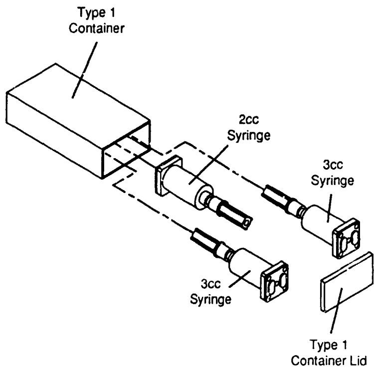
Figure 3. Fixative Syringes.
