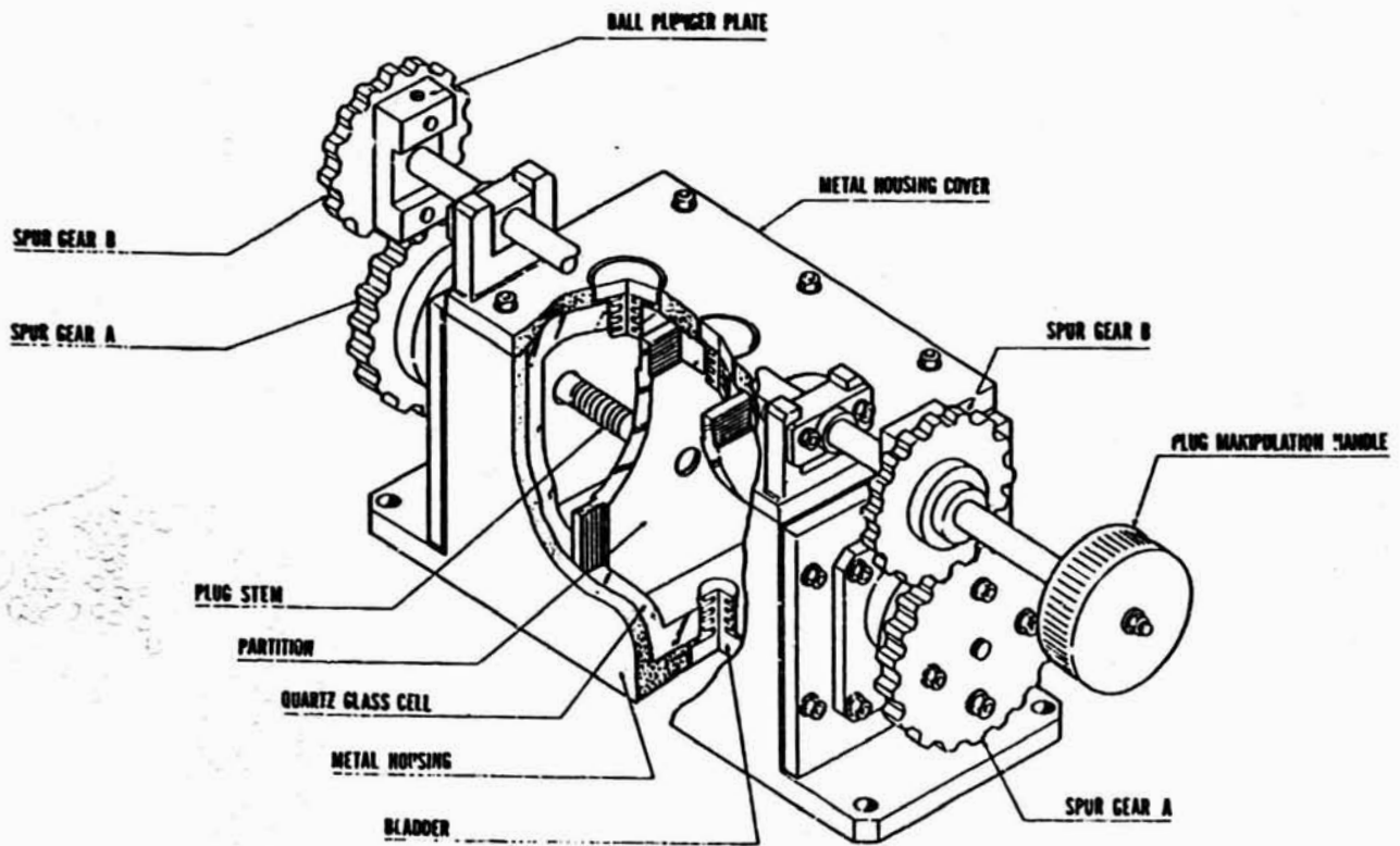
Figure 2b. Organic Crystal Growth Cell Flight Model.
