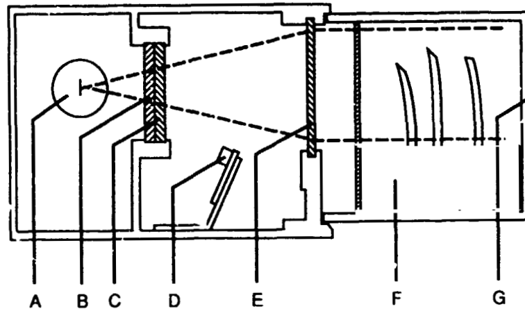
Figure 5. Section through the stimulus light source with growth container in position. A, Tungsten-filament bulb; B, lexan filter element; C, Corning blue glass filter, type 5433; D, photoresistor; E, Fresnel lens; F, seed tray with photostimulus window; G, growth-container body.
