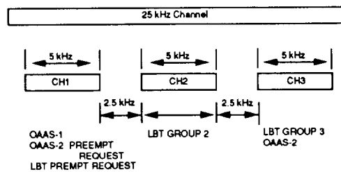
Figure 3 FREQUENCY ALLOCATIONS
