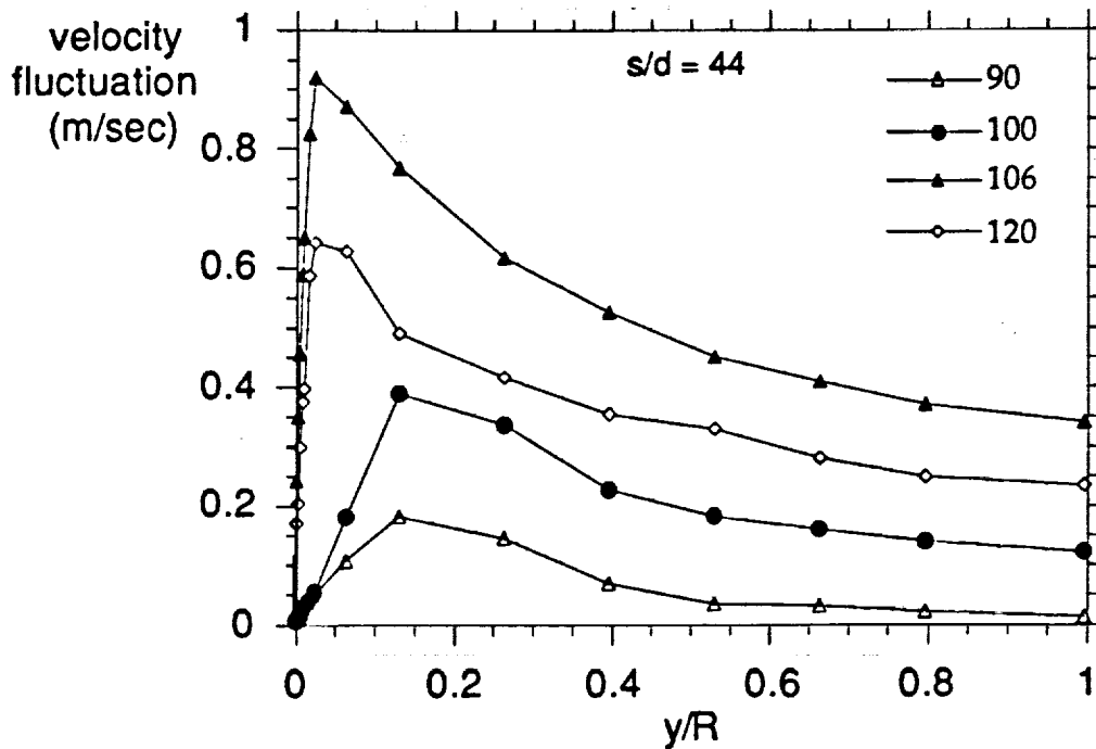
Figure 69: Profiles of streamwise velocity fluctuation at s/d = 44 .
