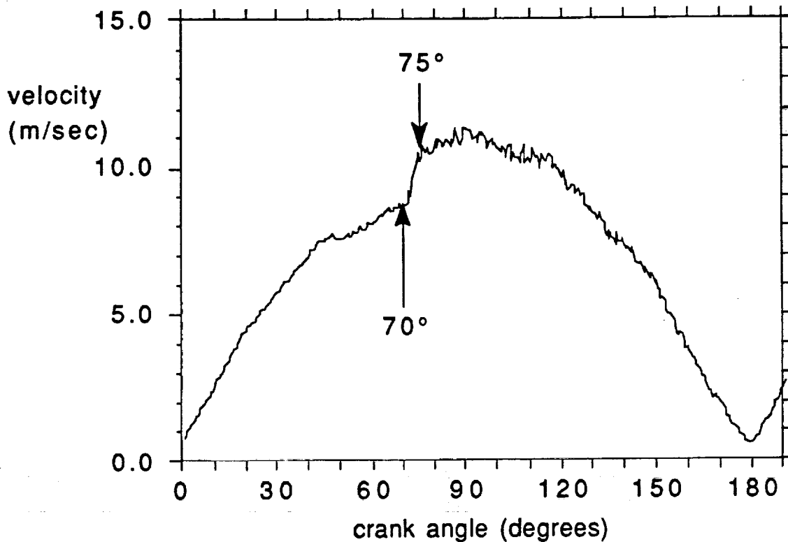
Figure 39: Ensemble-averaged velocity trace near the drive end case 1 x/d = 8.33 , l/d = 60 r/R = 0.96 , and y/d = 0.02 .
