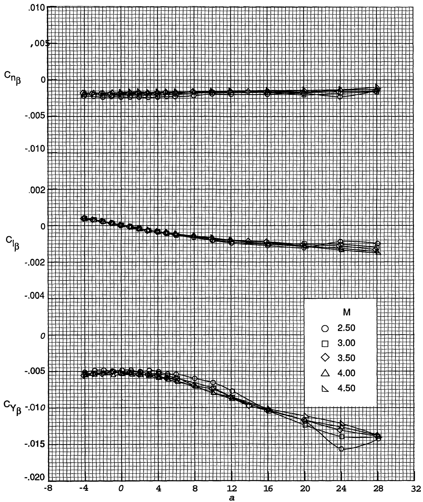
Figure 23. Effect of Mach number on lateral-directional stability derivatives, W1BN5.
