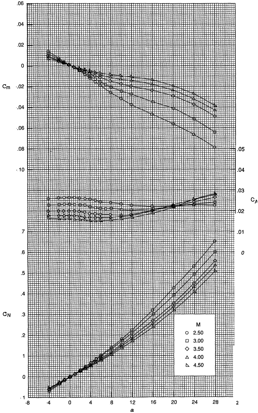
Figure 8 Effect of Mach number on longitudinal aerodynamic characteristics; W113N5V1
