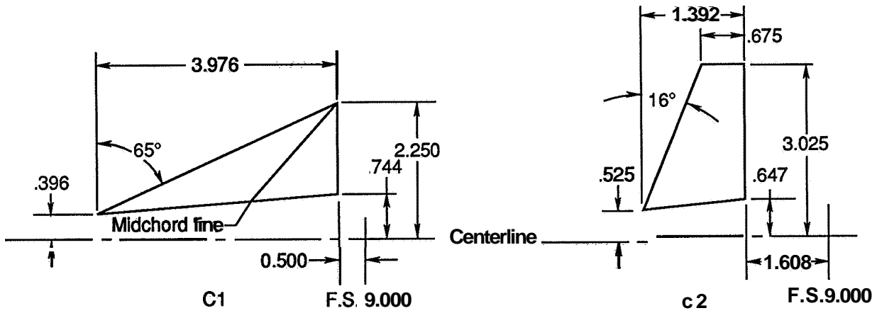
(c) Canard details.
