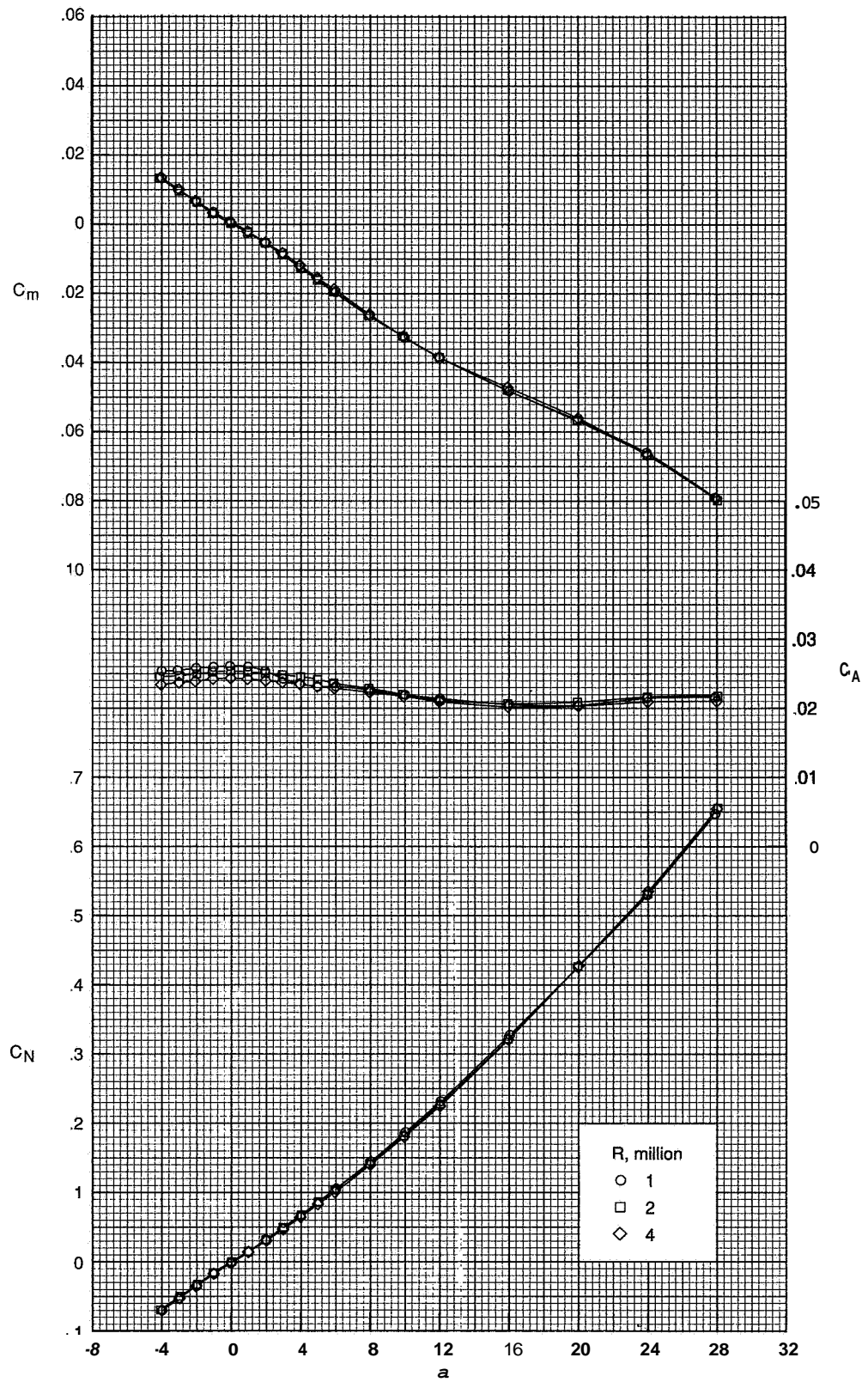
Figure 4 Effect of Reynolds number on longitudinal aerodynamic characteristics; W1BN5; M = 2.50
