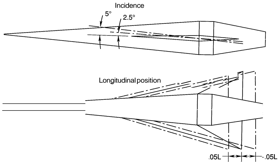
(f) Wing incidence and position variables.
