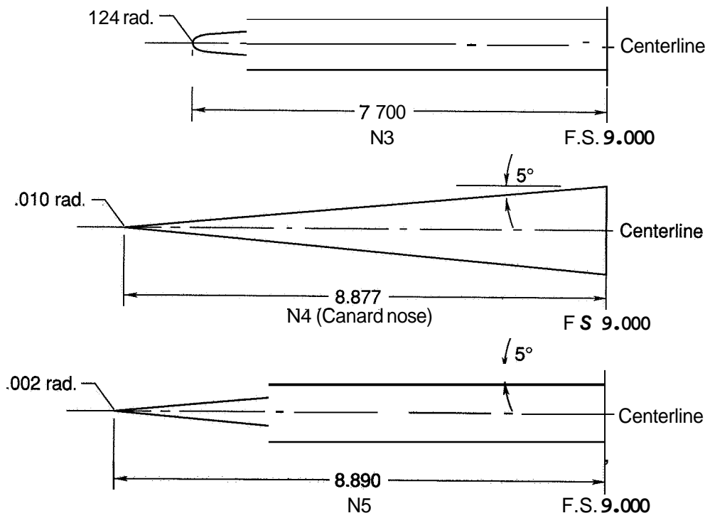
(b) Details of the fuselage nose.
