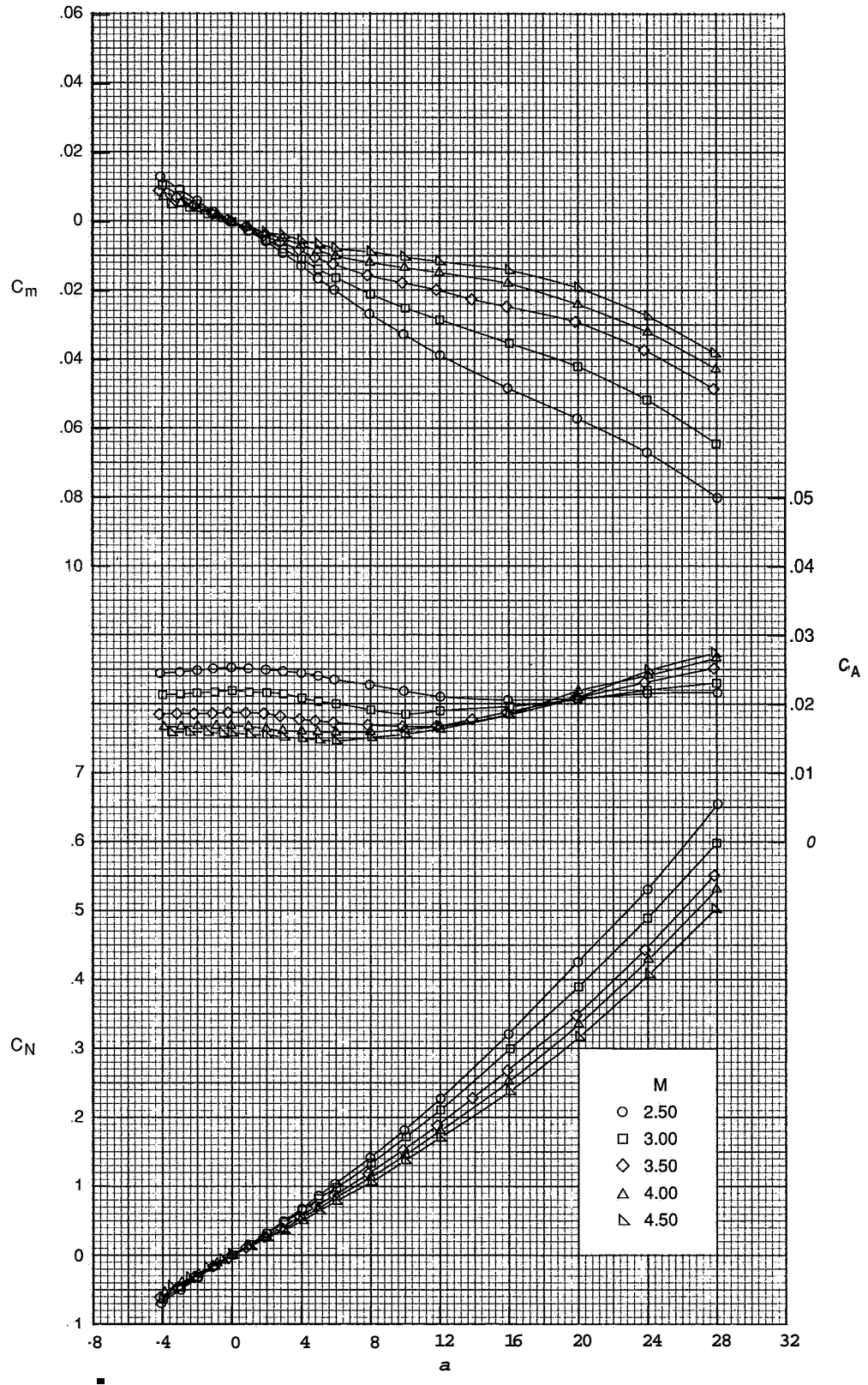
Figure 7 Effect of Mach number on longitudinal aerodynamic characteristics; W1BN5.
