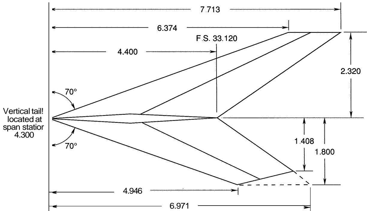
(e) Details of wing-mounted vertical tail
