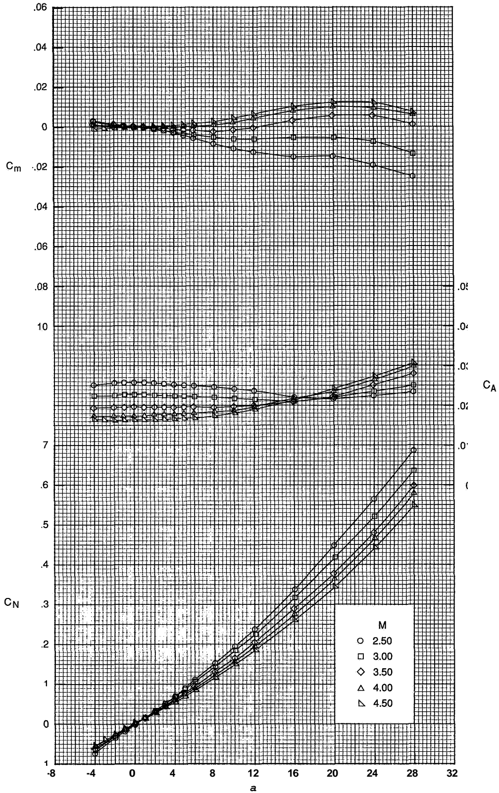
Figure 9. Effect of Mach number on longitudinal aerodynamic characteristics; W1BN4C1
