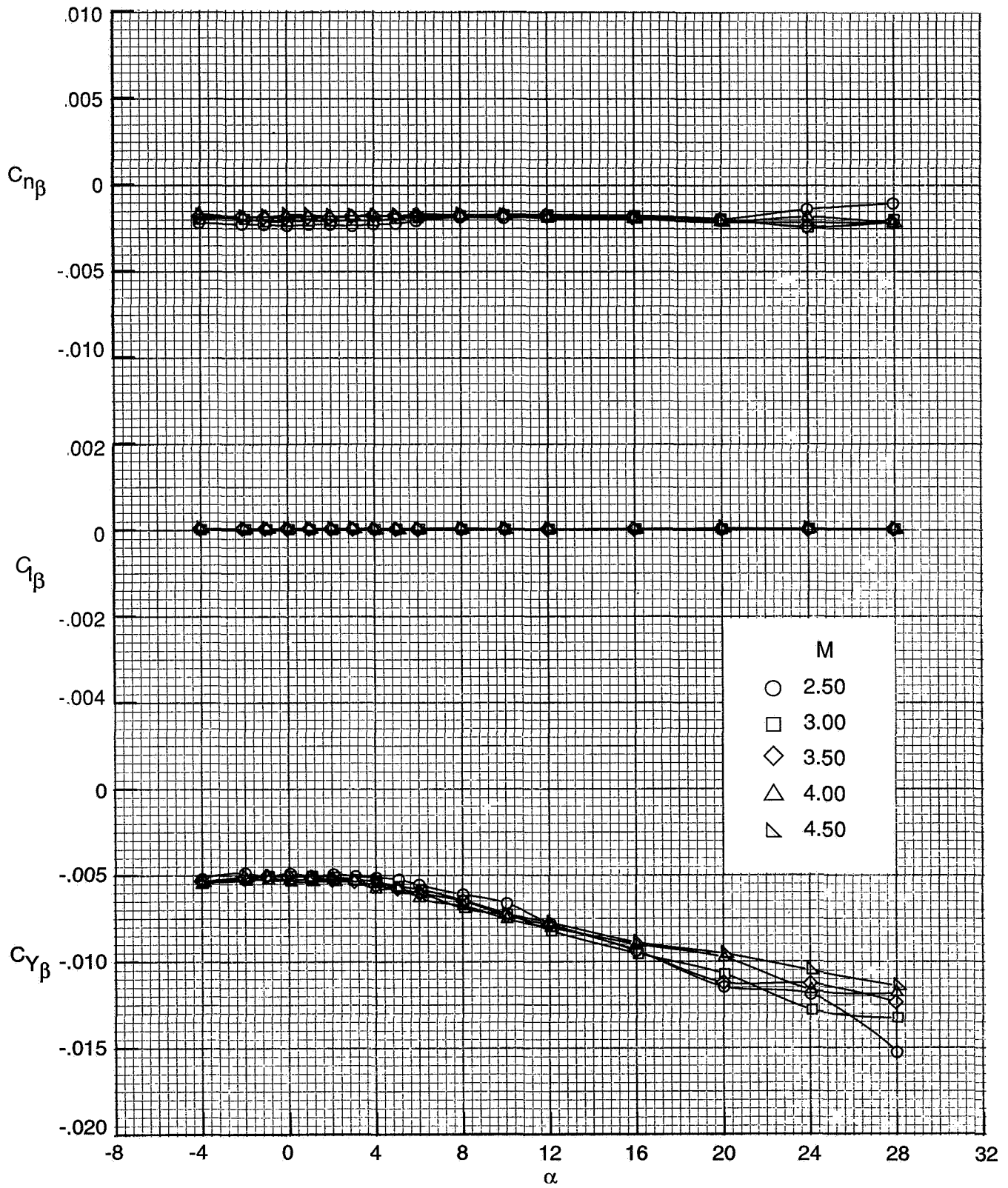
Figure 22 Effect of Mach number on lateral-directional stability derivatives; BN5
