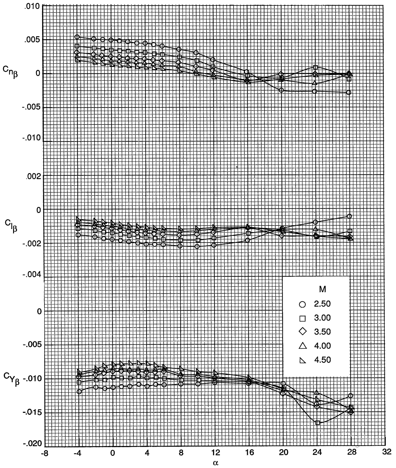
Figure 24. Effect of Mach number on lateral-directional stability derivatives; W1BN5V1
