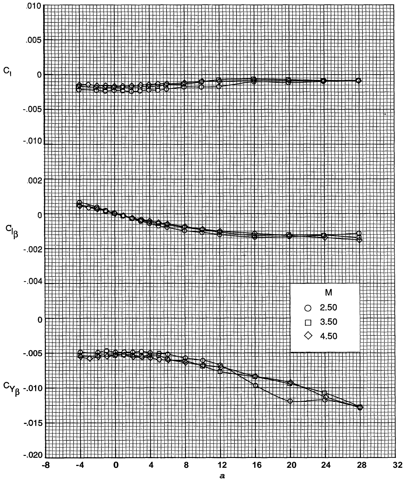
Figure 25 Effect of Mach number on lateral-directional stability derivatives, W1BN4C1
