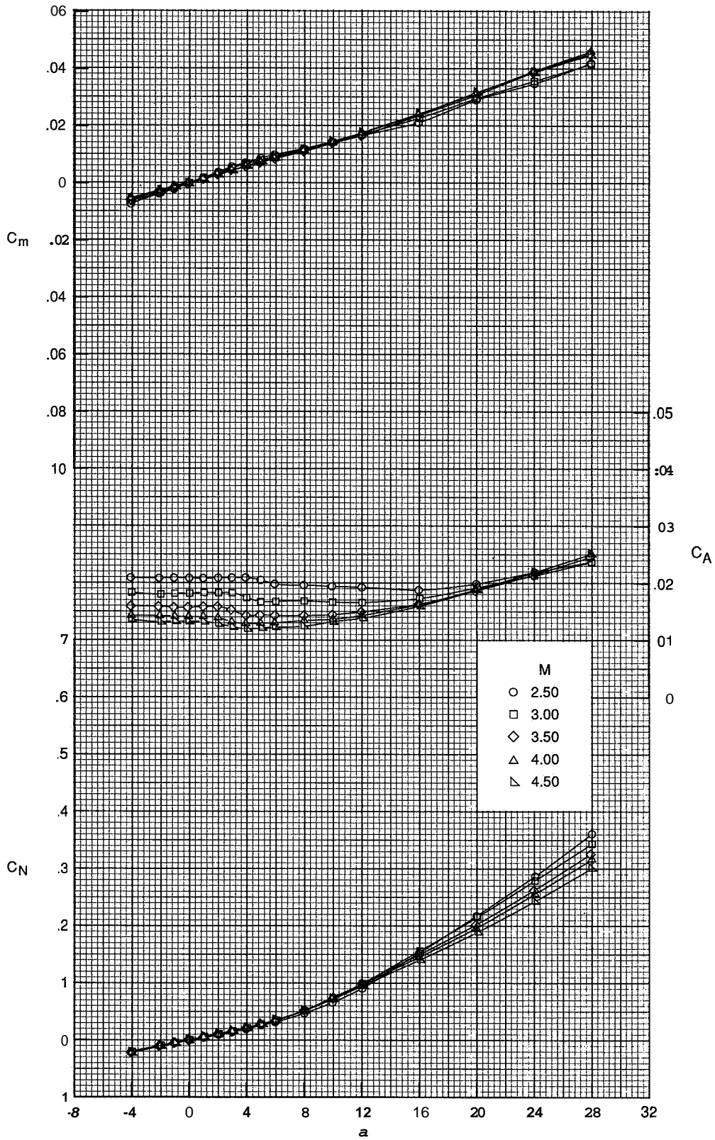
Figure 6. Effect of Mach number on longitudinal aerodynamic characteristics; BN5.
