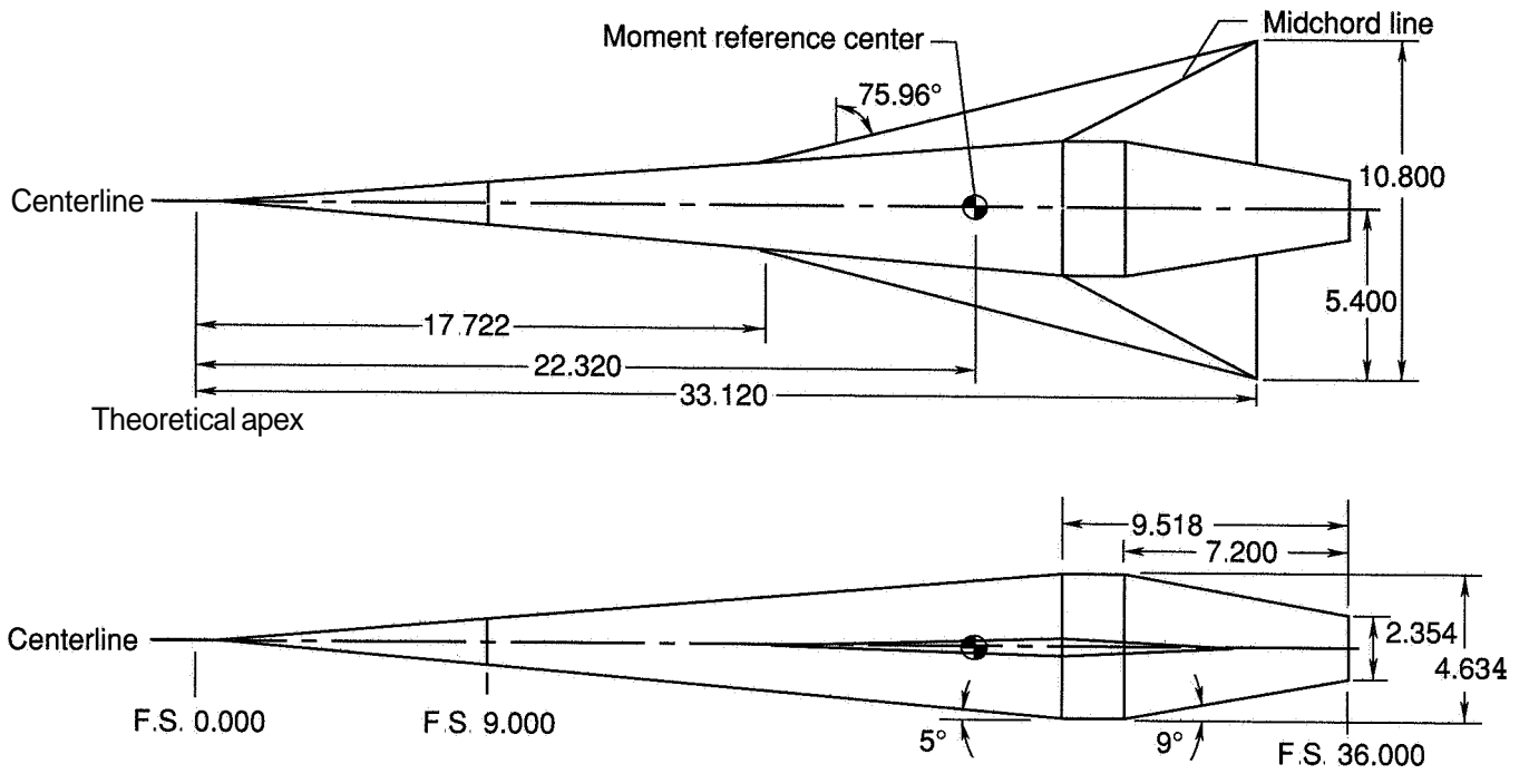
(a) General arrangement of the model. Wing in baseline (mid) position at zero incidence
