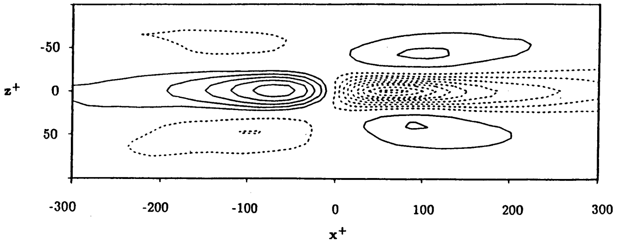
Figure 12. Contours of conditionally averaged velocities in fully developed turbulent channel flow. (a) Streamwise velocity in the x - y -plane along the centerline. (b) Streamwise velocity in the x - z -plane at y^+ = 15 . The mean flow direction is from left to right, cont. spacing 0.5u_\tau .
