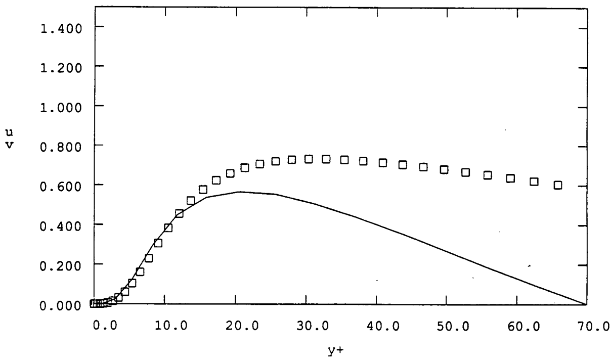
Figure 9. Comparison of normal dependence of turbulence quantities from the turbulent part of the spot (lines) with results from Kim, Moin, & Moser (1987), (symbols). (a) R.m.s. velocities, ( \square : u , \nabla : v , \diamond : w ) (b) Reynolds stress, normal coordinate in wall units,
