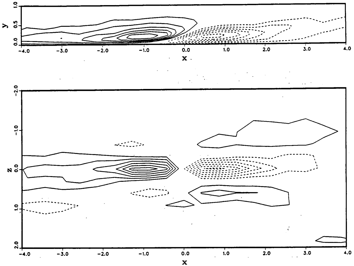
Figure 11. Contours of conditionally averaged velocities in the turbulent area. (a) Streamwise velocity in the x-y -plane along the centerline. (b) Streamwise velocity in the x-z -plane at y = 0.78 . The mean flow direction is from left to right, and the contour spacing is 0.025 or 0.5u_\tau .
