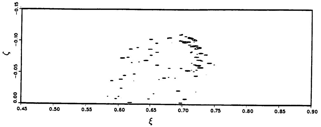
Figure 10. Islands of high variance obtained using the VISA technique, y^+ = 12 . Contour spacing k = 0.5 , no zero contours plotted.
