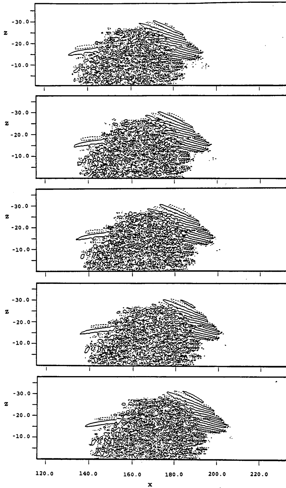
Figure 6. Time development of the instantaneous normal velocity at the centerline, \pm 0.01 contours at (a) t = 246 , (b) t = 249 , (c) t = 252 , (d) t = 255 , (e) t = 258 .
