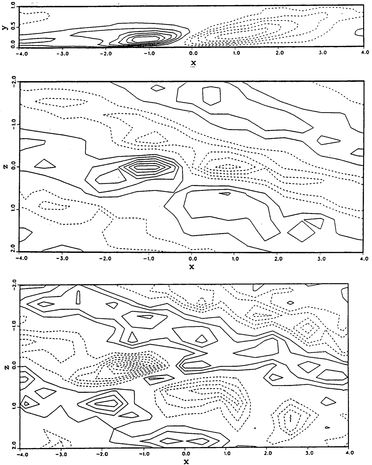
Figure 13. Contours of conditionally averaged velocities in the wave area. (a) Streamwise velocity in the x - y -plane along the centerline. (b) Streamwise velocity in the x - z -plane at y = 0.78 . (c) Normal velocity in the x - z -plane at y = 0.78 . The mean flow is from left to right. The the contour spacing for (a) and (b) is the same as in fig. 11, and for (c) is 0.005 or 0.1u_\tau .
