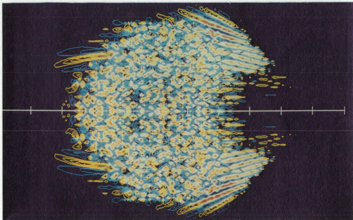
Figure 1. Contours of instantaneous velocity at t = 258 of (a) streamwise velocity at y = 0 (blue, green, yellow, orange, red to pink indicate a velocity range of 0.5 to 1.15, with orange being about unity); (b) normal velocity at y = 0 (light to dark blue indicates a velocity range from 0.0 to 0.15 in the negative y -direction whereas yellow to red indicates a velocity range from 0.0 to 0.15 in the positive y -direction).
