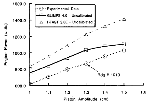
Figure 3 - RE-1000 Engine Power vs Piston Amplitude (Uncalibrated Predictions)
