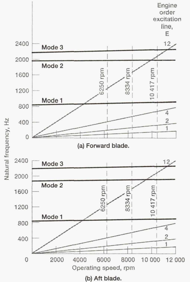
Figure 12.—CM-1C Campbell diagrams.
