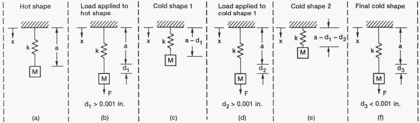
Figure 9.—Schematic of cold shape iteration.
