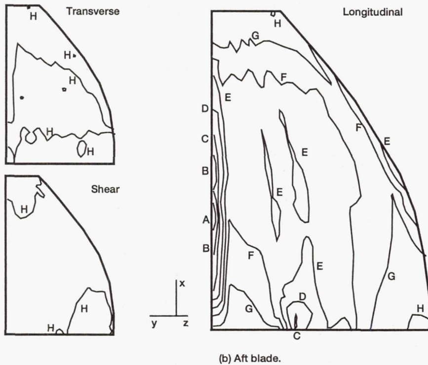
Figure 14.—CM-1D stress plots; pressure side.
