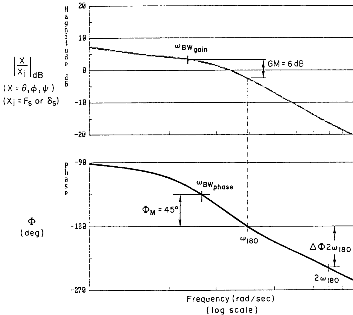
Figure 20. Definitions of Bandwidth and Phase Delay
