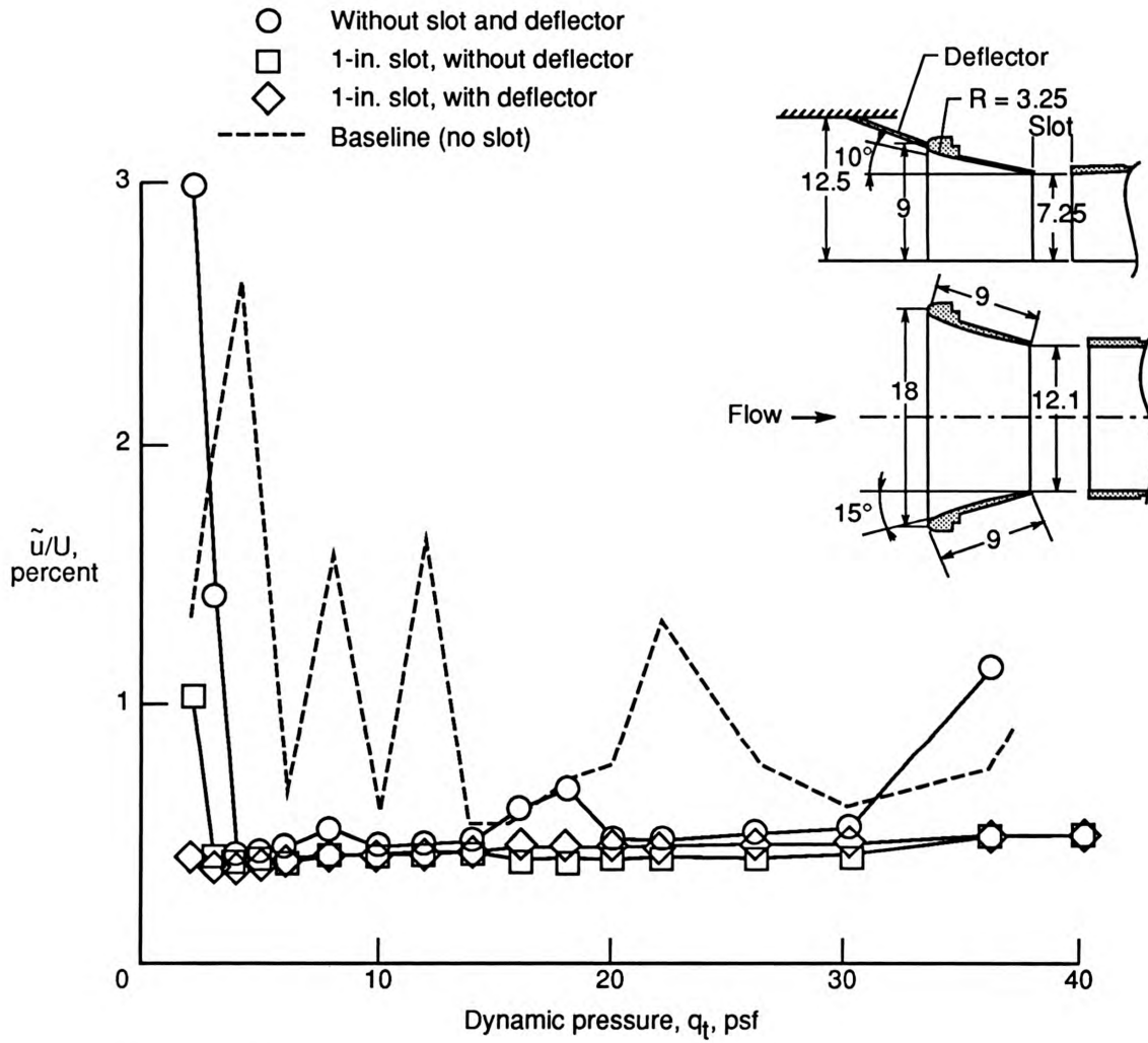
Figure 6. Effect of deflector and slot on test section turbulence for configuration 2.
