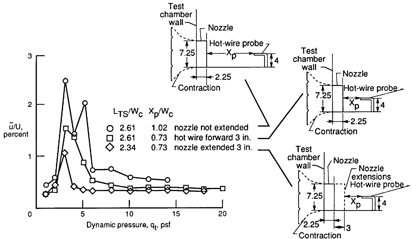
(b) Nozzle extensions and hot-wire probe locations.
