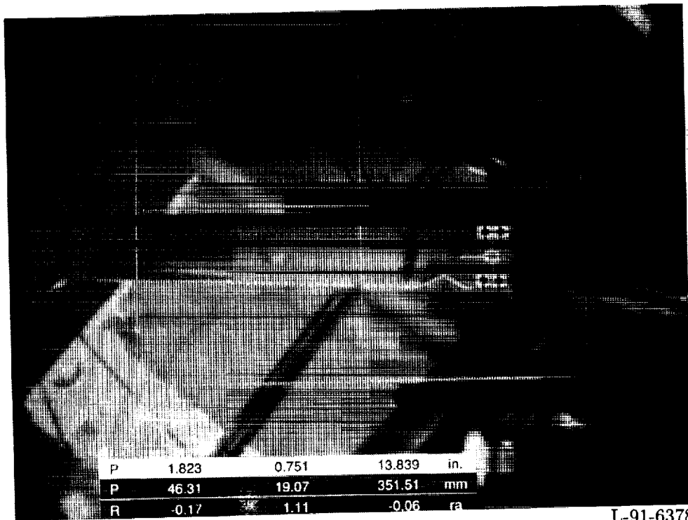
(g) Processed image after target lock-on and pose estimation. Top two lines of key give position vector in inches and millimeters, respectively. The bottom line gives rotation vector in radians.
