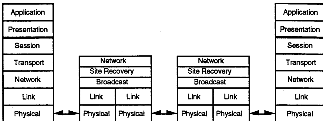
Figure C-3: Scientific Atlanta VSAT Protocol Architecture
