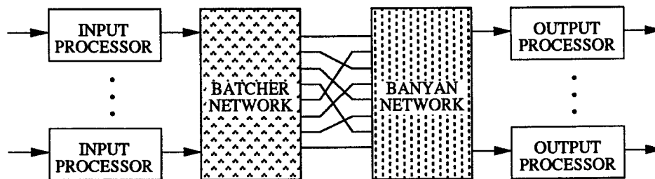
Figure 4-10: Sorted-Banyan Baseband Switch Structure
