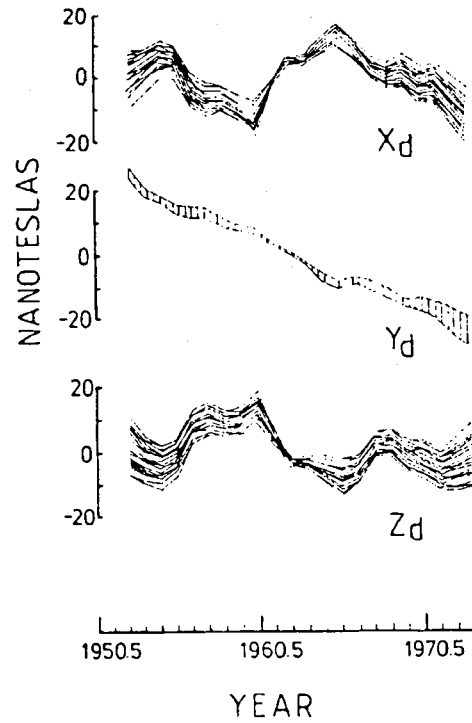
Fig. 3. Variation of the components of the external dipole field between 1952.5 and 1980.5.
