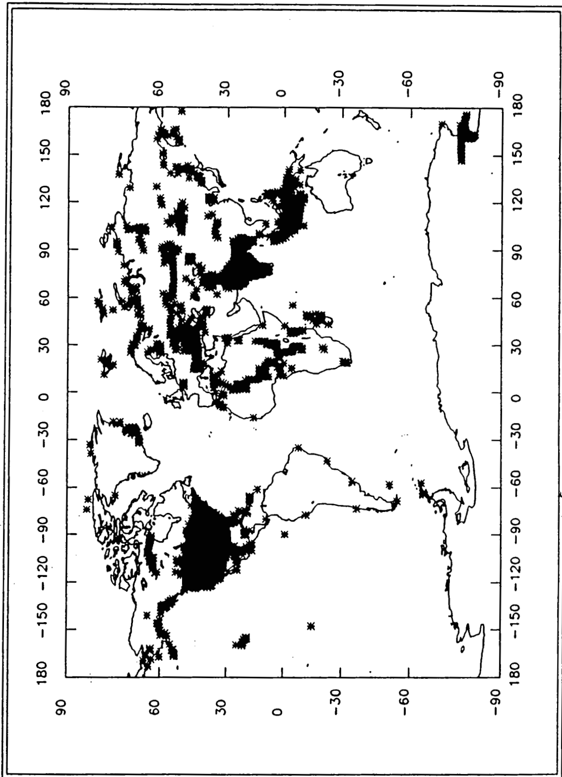
Figure 1. Positions of land survey data based on observations made between 1900.0 and 1907.5.
