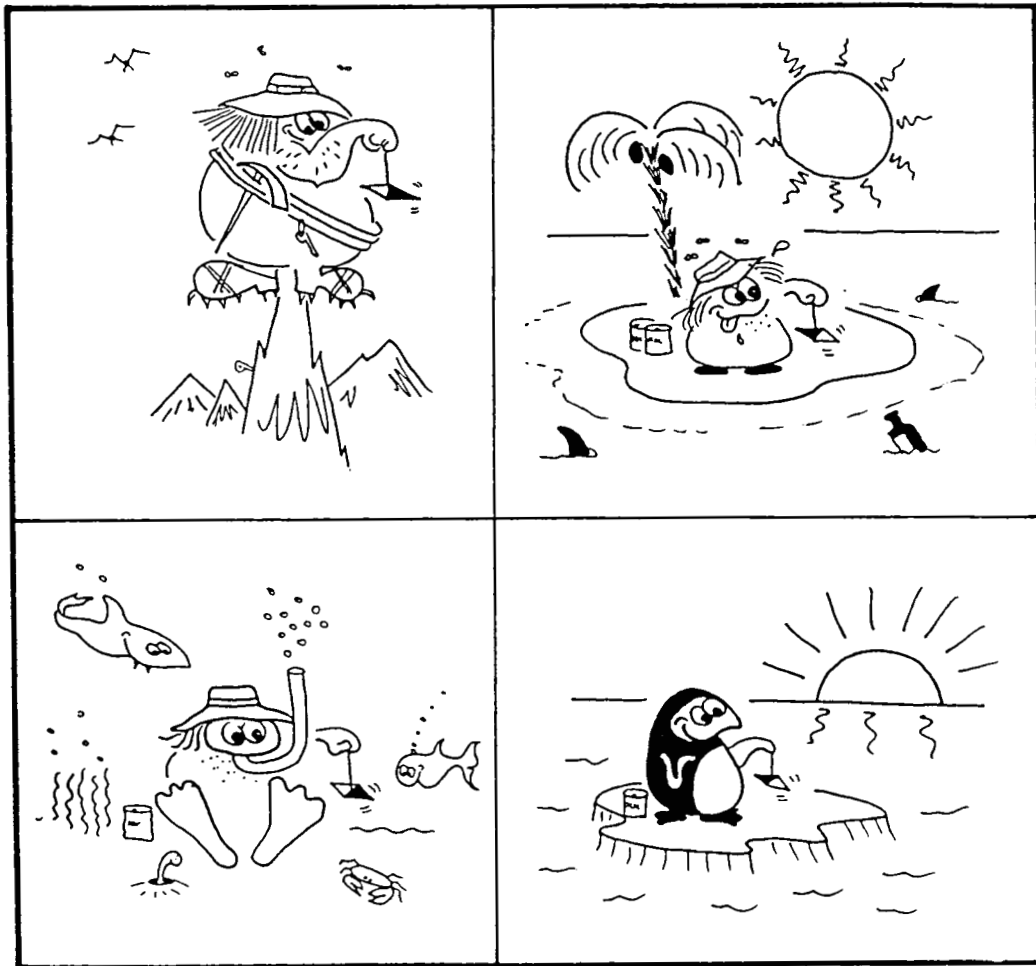
Figure 1. Repeat stations provide secular variation information where observatory coverage is inadequate.
