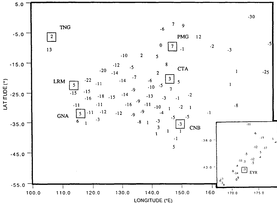
Figure 2. Differences in the annual change in Z for 1990.0 between repeat station estimates and IGRF90 (units of nT\ yr^{-1} ). Boxed values are (observatory - IGRF90) differences. The region covers Australia, Papua New Guinea, Islands in the SW Pacific and New Zealand (inset, expanded to double scale). Observatory codes are: CNB = Canberra, CTA = Charters Towers, EYR = Eyrewell, GNA = Gnangara, LRM = Learmonth, PMG = Port Moresby, TNG = Tangerang. (Data provided by Andrew McEwin and Don McKnight).
