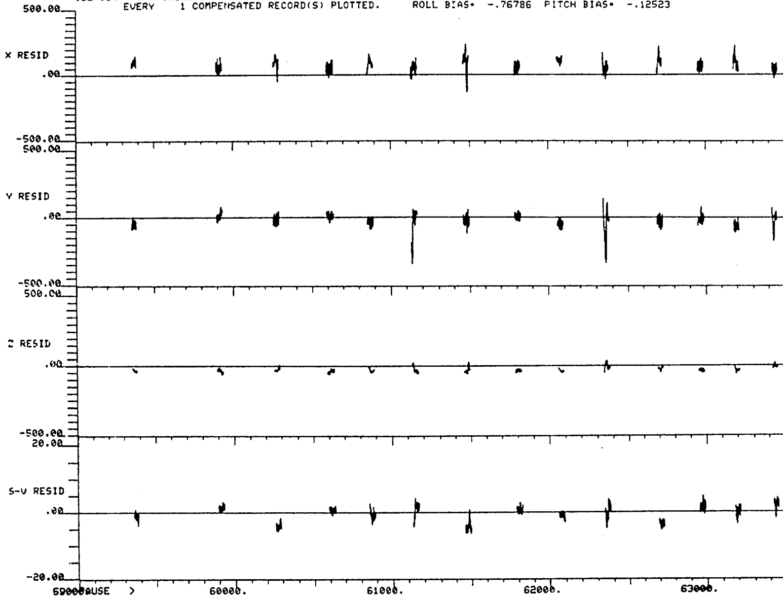
Figure 7. College, Alaska Geomagnetic Observatory Residual Plots.
