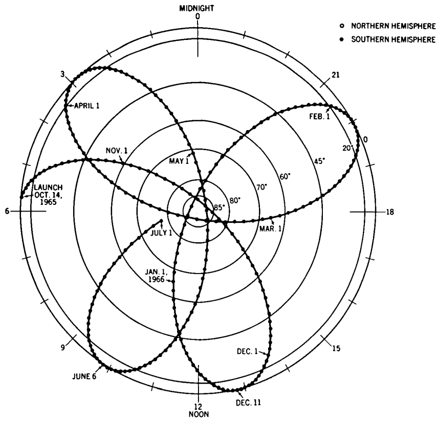
PERIGEE MOTION OF POGO-1 ORBIT OCT. 14, 1965 - JULY 1, 1966
