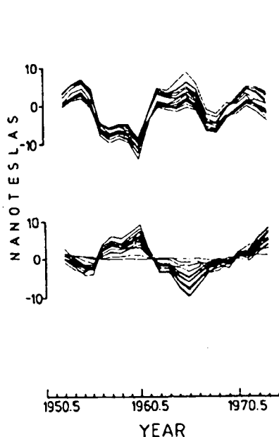
Fig. 4. Induction model. Calculated \Delta H_s and \Delta Z_s .
