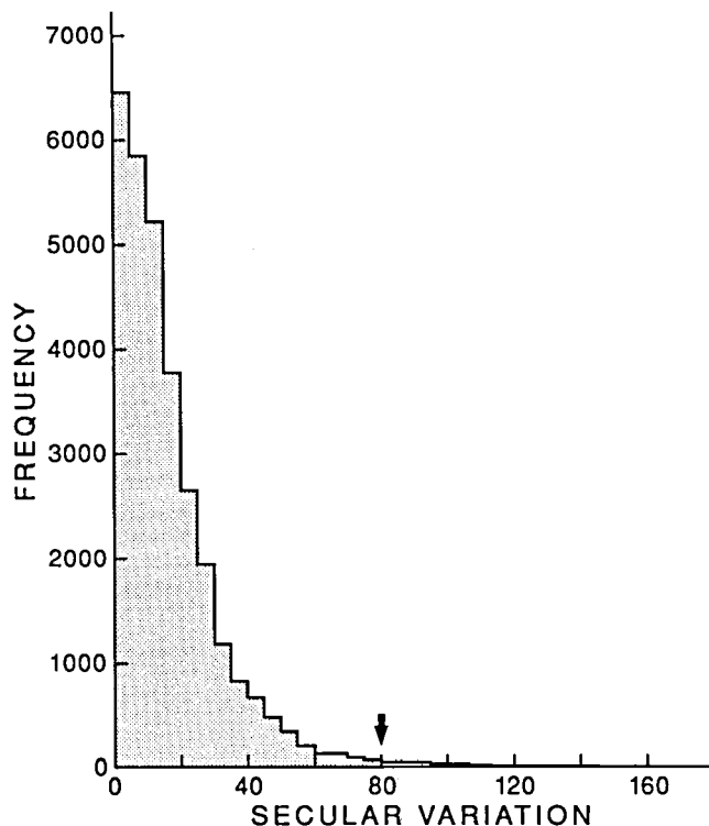
Fig. 3. Frequency distribution of the observed secular variations obtained at the crossover points shown in Fig. 1. 80 nT was used as a cutoff value for eliminating crossovers that indicated unrealistically high secular variations.
