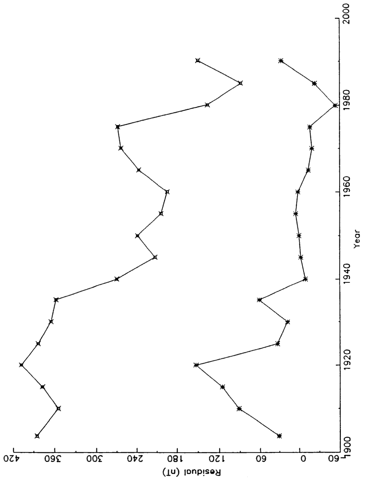
Figure 24. Mean and root mean square residuals between observed and computed values for each of the 18 time windows.
