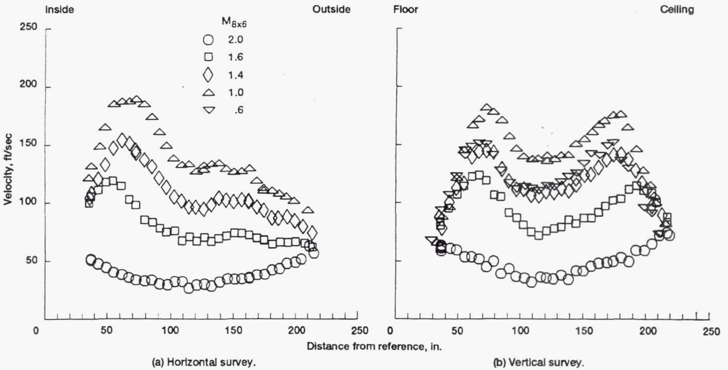
Figure 27.—Velocity distributions in settling chamber upstream of 8- by 6-ft test section from hot-film anemometry data.
