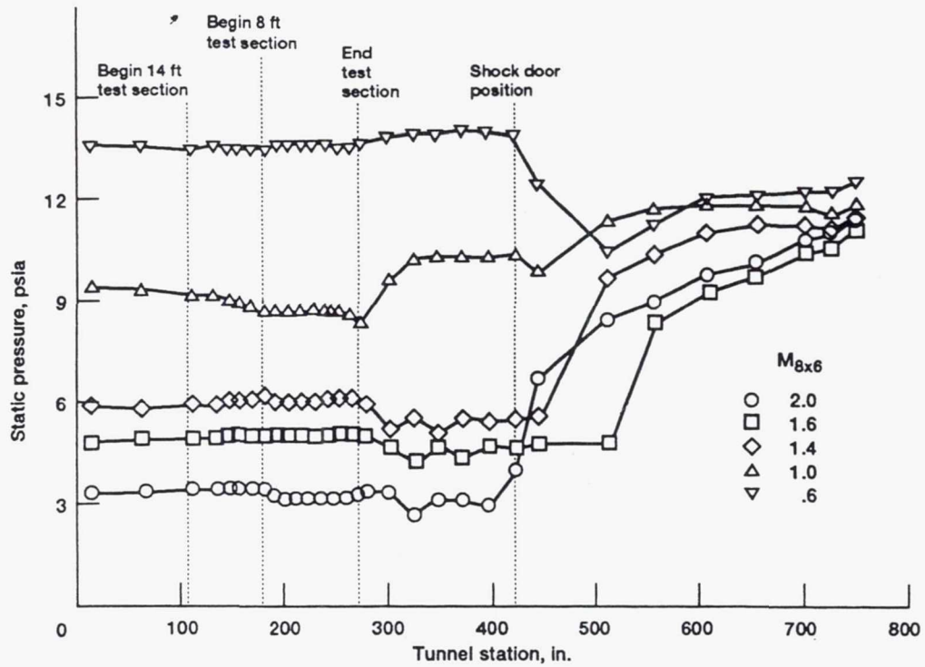
Figure 38.—Ceiling static pressure distribution through 8- by 6-ft test section and forward diffuser section.
