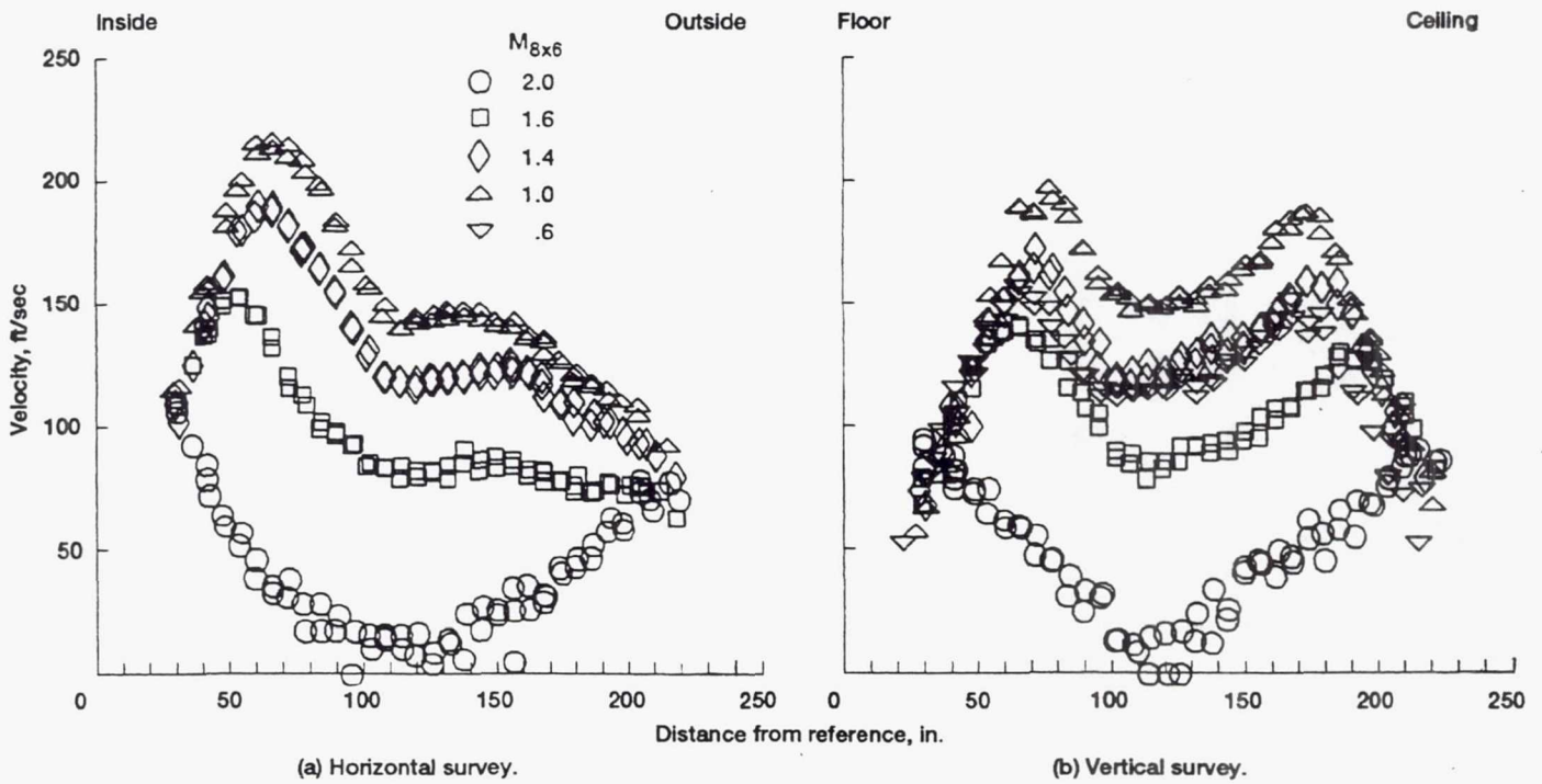
Figure 26.—Velocity distributions in settling chamber upstream of 8- by 6-ft test section from pitot-static probe data.
