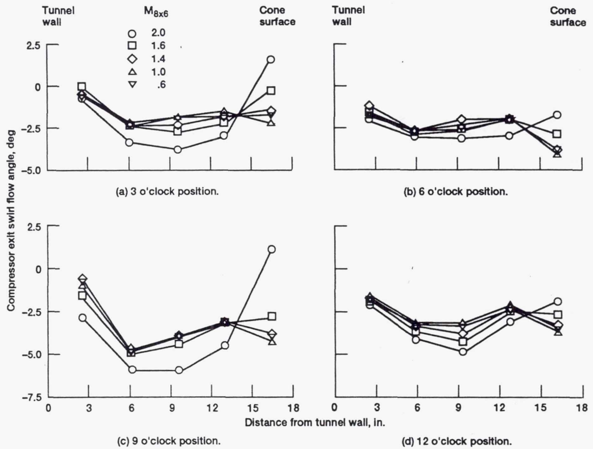
Figure 21.—Swirl flow angularity data at compressor exit (negative in direction of compressor rotation).
