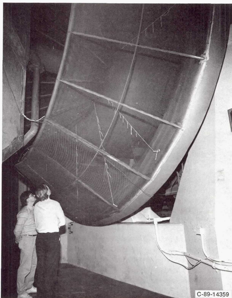
Figure 4.—Inlet to seven-stage axial flow compressor showing flow visualization tufts (view is north side of inlet).
