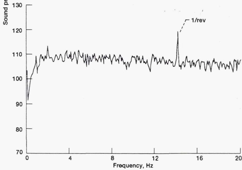
(b) Rotor 2.
