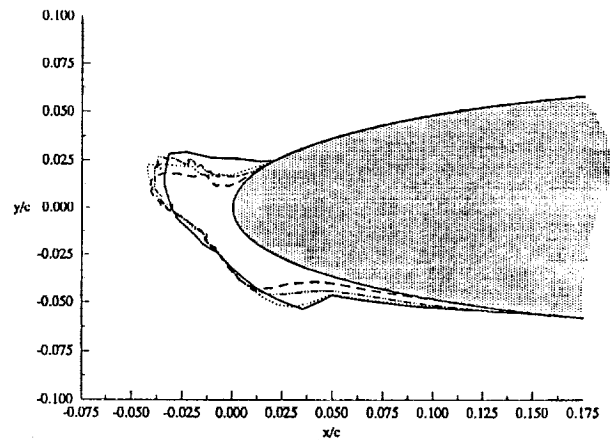
(b) AOA=4^\circ , V_\infty=150 mph, T_T=18^\circ\text{F} , LWC=1.0\text{g/m}^3 , MVD=20\mu\text{m} , Accretion Time = 6 min.
