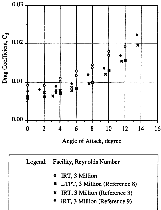
Fig. 3. Comparison of Measured Clean Airfoil Drag with Published Data for the NACA 0012 Airfoil.
