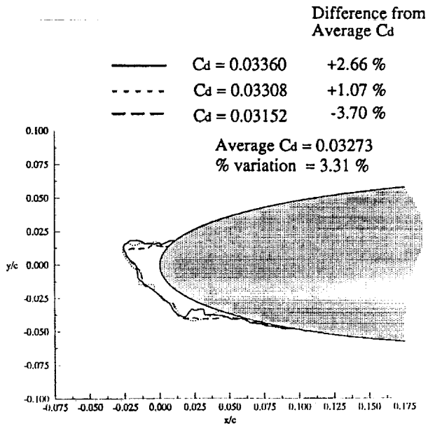
(a) AOA=4^\circ , V_\infty=150 mph, T_T=22^\circ F , LWC=1.0g/m^3 , MVD=20\mu m , Accretion Time = 6 min.
