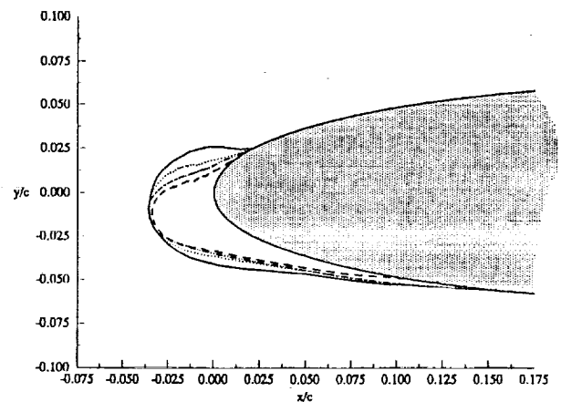
(c) AOA=4^\circ , V_\infty=150 mph, T_T=-15^\circ\text{F} , LWC=1.0\text{g/m}^3 , MVD=20\mu\text{m} , Accretion Time = 6 min.
