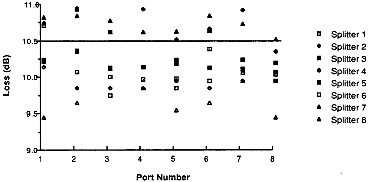
Figure 3-2. Loss map for Corning splitters.
