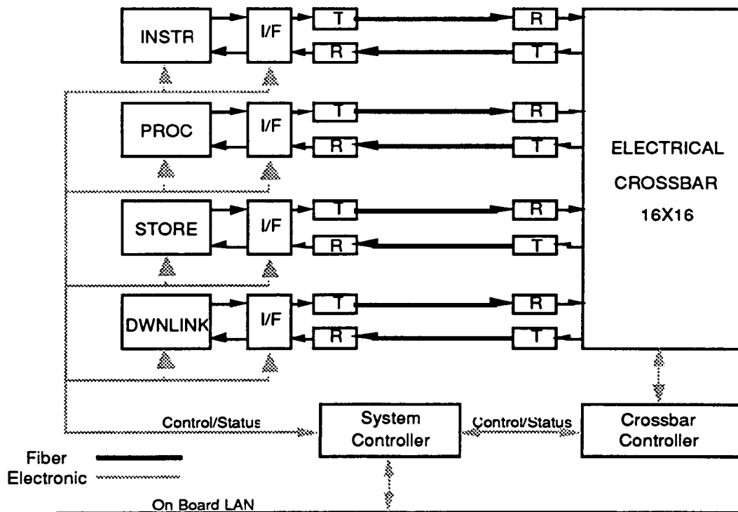
Figure 1-6. Generic on-platform electrical crossbar implementation.
