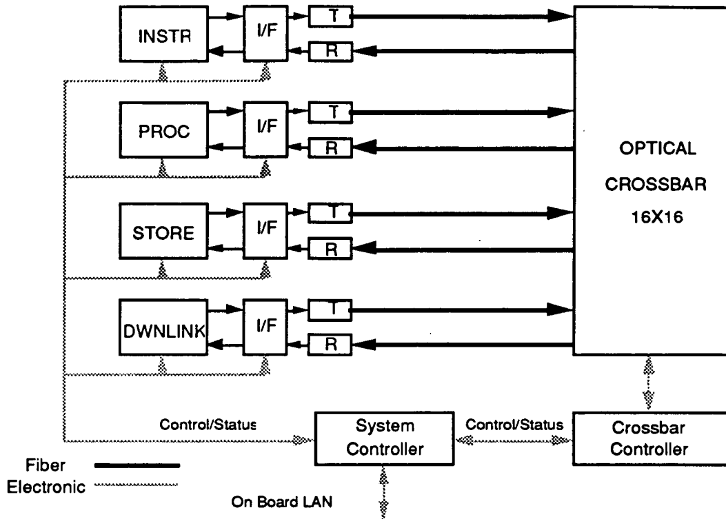
Figure 1-5. Generic on-platform optical crossbar implementation.
