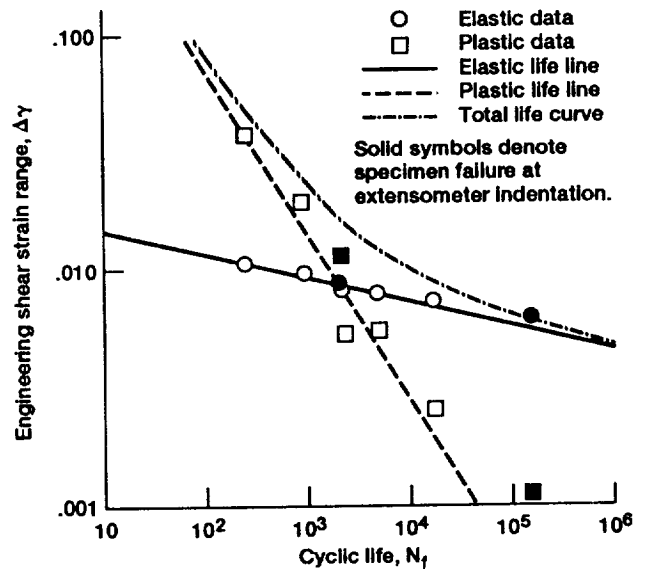
Figure 10.—Torsional fatigue life relations for Haynes 188 at 760 °C.
