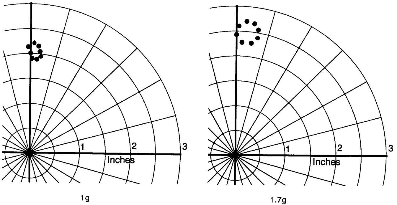
Figure 4. Effect of Gravitational Strength on Particle Path.
