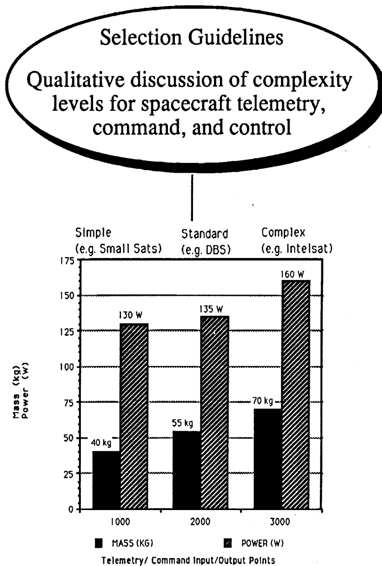
Figure 1-8: Telemetry, Tracking and Command (TT&C) Sizing and Selection Guidelines
