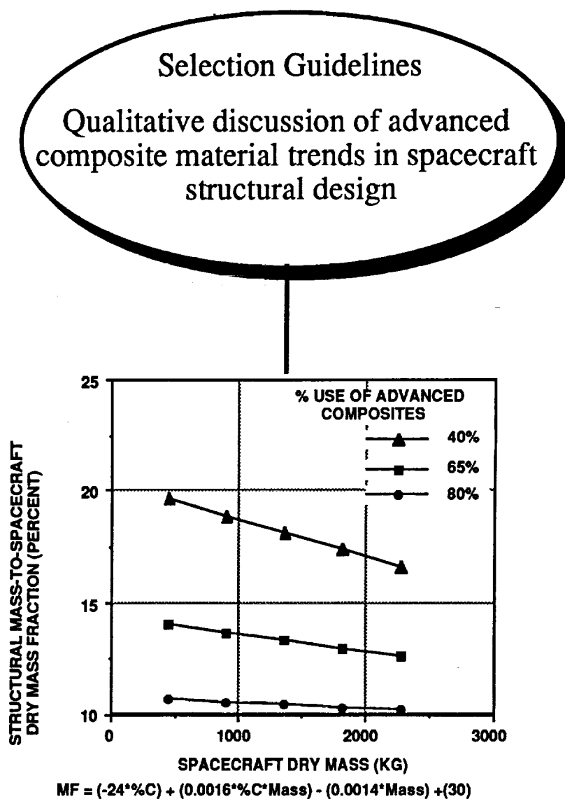
Figure 1-6: Structural Sizing and Selection Guidelines
