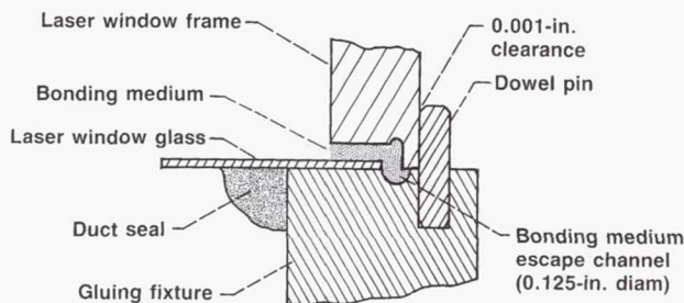
Figure 16.—Cross section of laser window bonding process.
