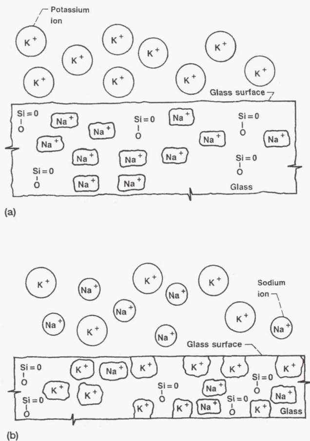
(a) Preceding ion exchange. (b) Subsequent ion exchange.
