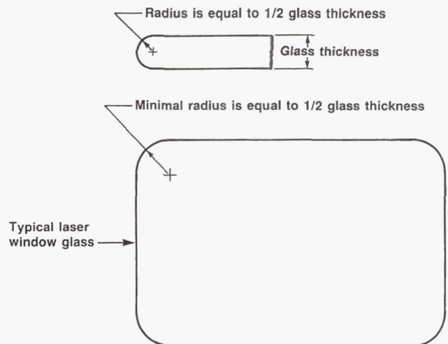
Figure 10.—Rounded edges of typical laser window.
