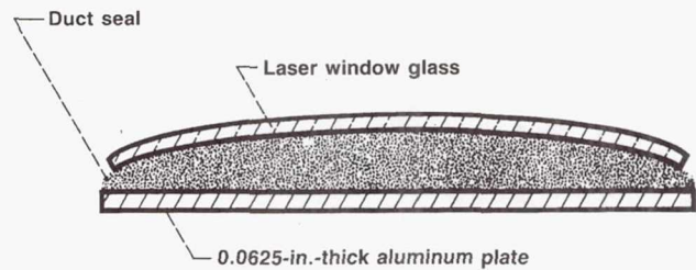
Figure 9.—Cross section of laser window edging process.
