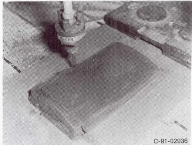
Figure 8.—Laser window glass positioned for edging in numerically controlled water-jet cutting machine.
