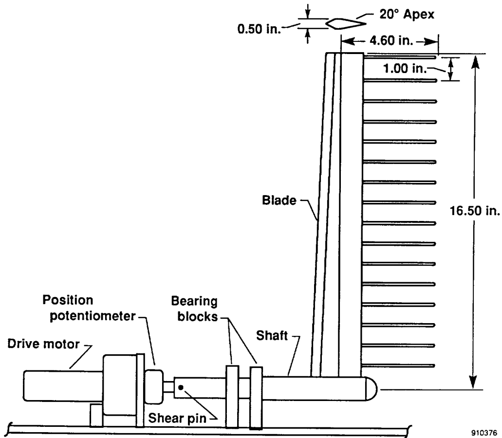
(c) Survey rake.
