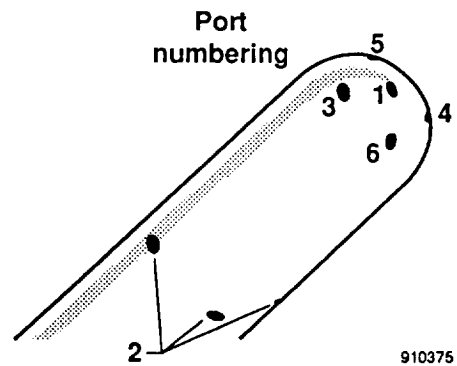
(b) Five-hole probe nomenclature.
