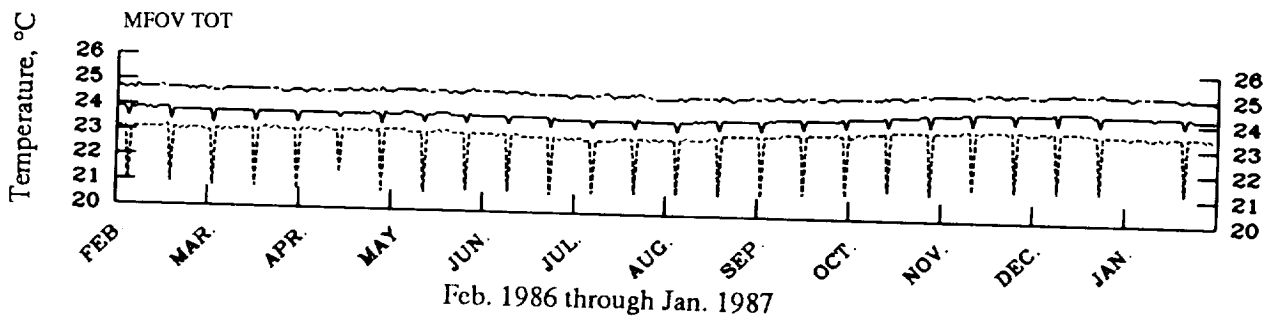
(c) Field-of-view limiter temperatures. Earth-viewing detectors.
