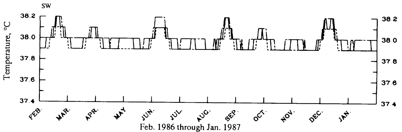
(a) Detector temperatures.
