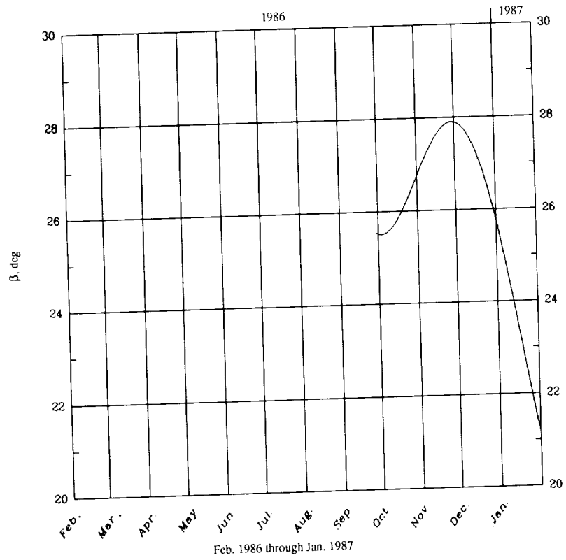
(c) NOAA 10 spacecraft for February 1986 through January 1987.
