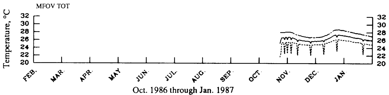
(c) Field-of-view limiter temperatures. Earth-viewing detectors.
