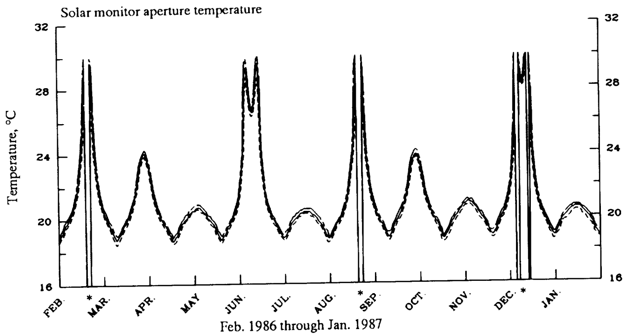
(d) Solar monitor heat sink and aperture temperatures. Asterisks (*) denote that all data exceeded maximum telemetry edit limits.
