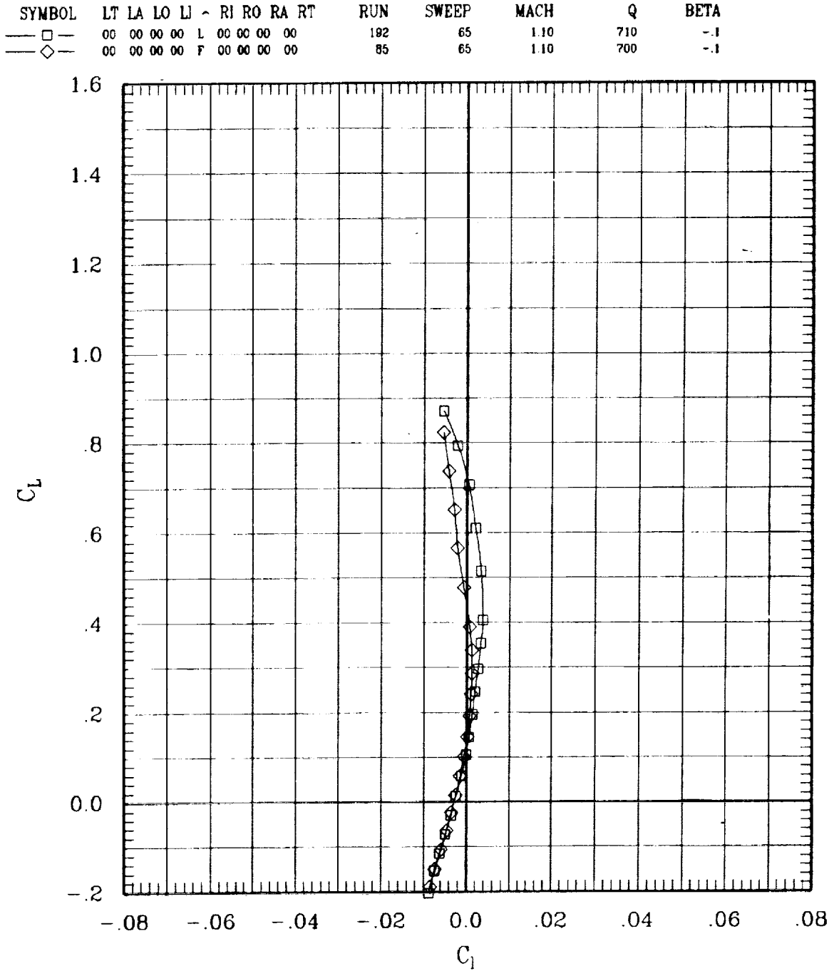
Figure 6(e). Effect of pivot height for sweep = 65 deg.
