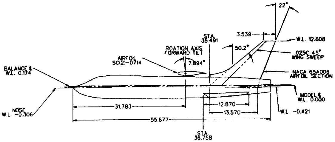
Figure 2. F-8 model with Rockwell oblique wing.
