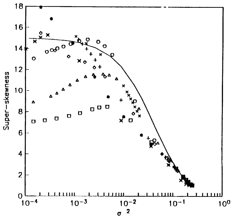
Figure 2: (a) HCS scalar flatness-factor vs. scalar variance and (b) scalar super-skewness vs. scalar variance, for the case of \mu = 0.5 . ( \square k_s = 1 ; \triangle k_s = 2 ; \circ k_s = 4 ; \diamond k_s = 6 ; + k_s = 8 ; * k_s = 10 ; \times k_s = 12 ; \blackstar k_s = 16 ; solid-line \beta -pdf model.)
