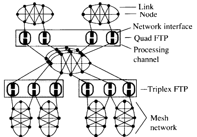
Figure 1. IAPSA architecture.
