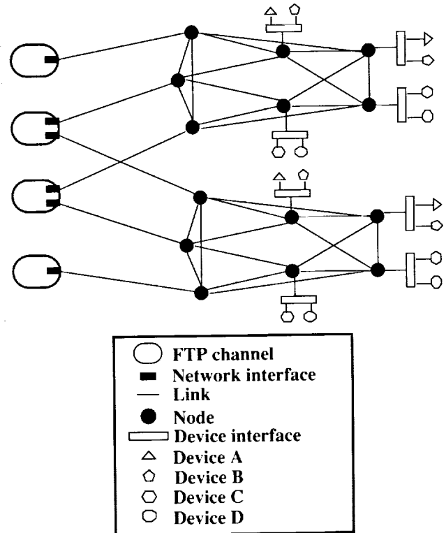
Figure 7. Example 3: Mesh network.
