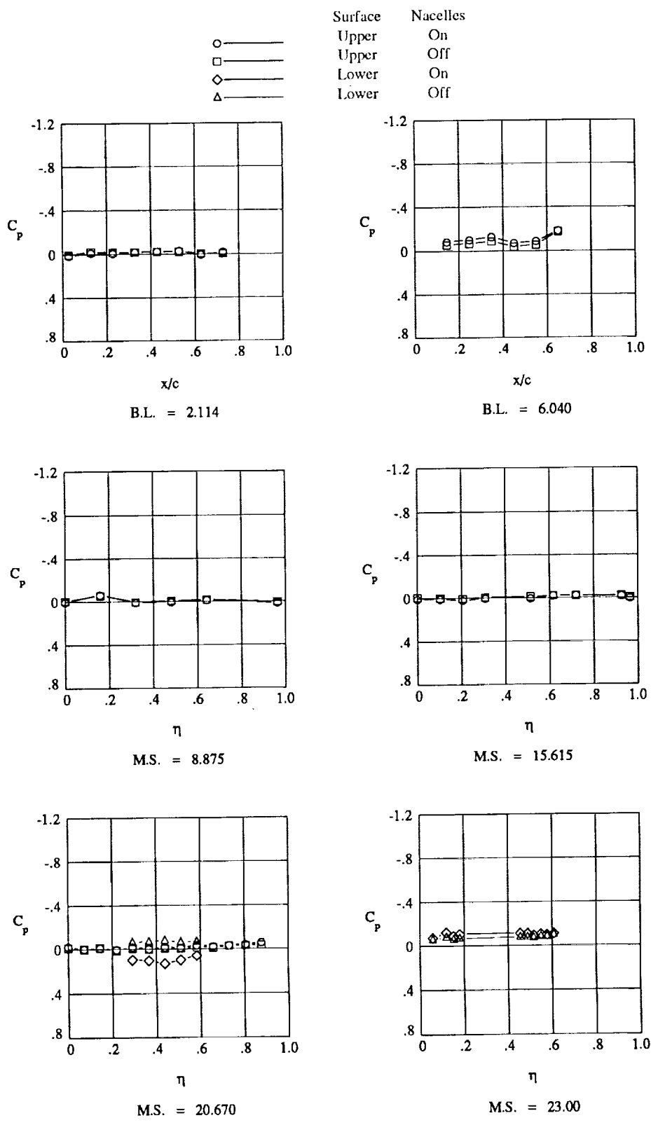
Figure 18. HSCT pressure distributions at M_\infty = 0.90 . Curved wingtip.
