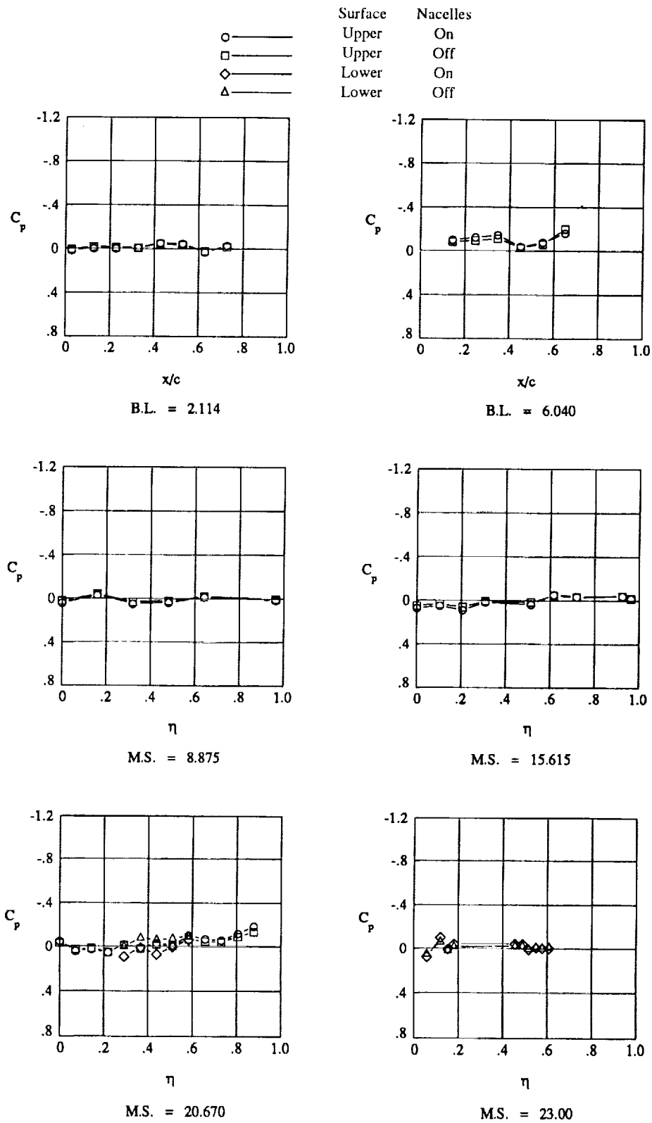
(b) \alpha = 0.04^\circ (nacelles on); \alpha = -0.23^\circ (nacelles off).
