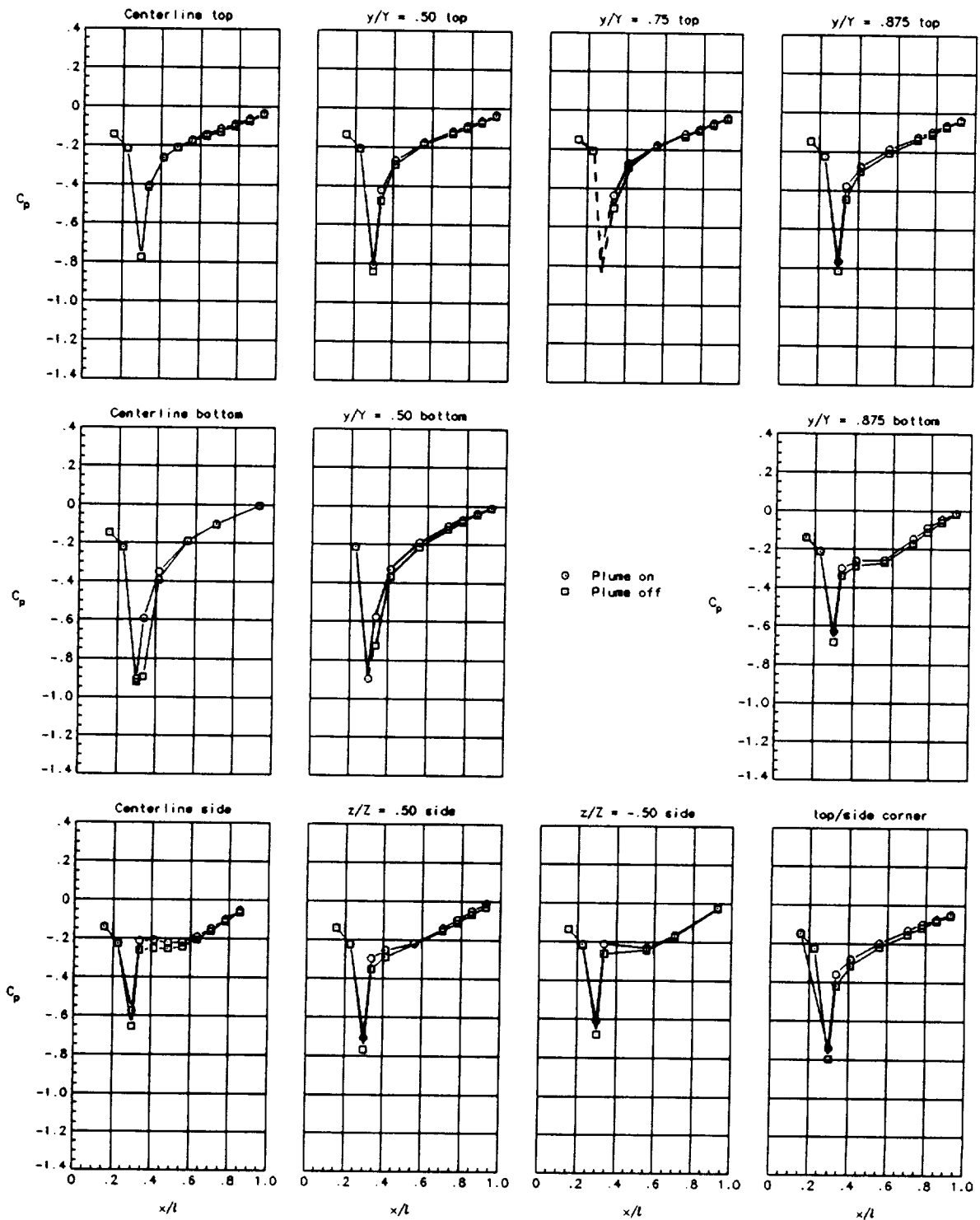
(q) Nozzle 8 with \beta_{t,top/bot} = 15.0^\circ / \beta_{t,side} = 22.4^\circ and 1-in. corner radius at M_\infty = 0.9 . C_{p,crit} = -0.188 .
