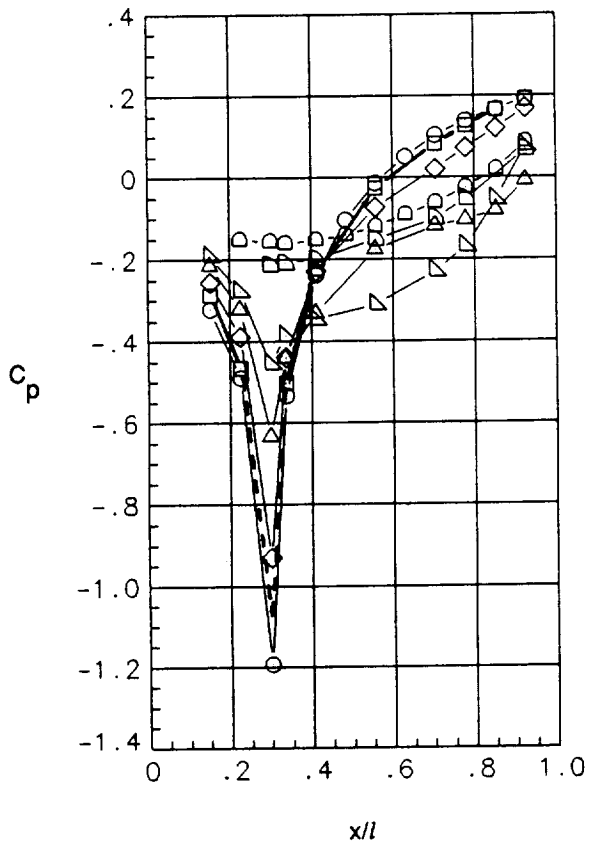
Nozzle 5: 1-in. corner radius
