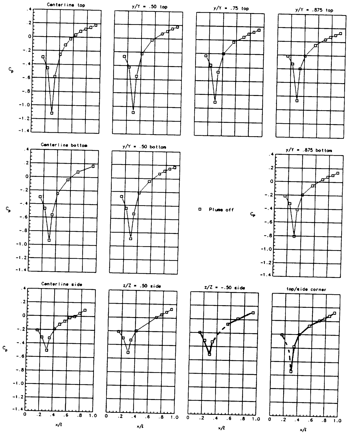
(k) Nozzle 6 with \beta_{t,top/bot} = 17.3^\circ / \beta_{t,side} = 9.7^\circ and 1-in. corner radius at M_\infty = 0.9 . C_{p,crit} = -0.188 .
