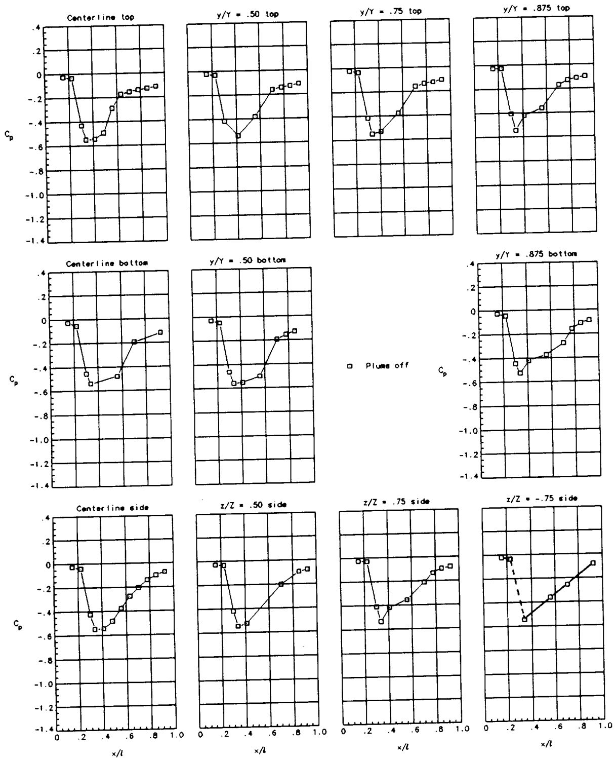
(f) Nozzle 3 with \beta_{t,top/bot} = 16.4^\circ / \beta_{t,side} = 16.4^\circ and sharp corner at M_\infty = 1.2 . C_{p,crit} = 0.279 .
