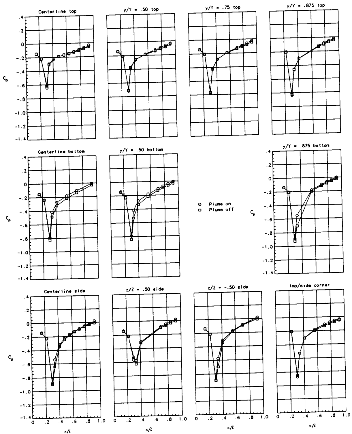
(n) Nozzle 7 with \beta_{t,top/bot} = 16.4^\circ / \beta_{t,side} = 16.4^\circ and 1-in. corner radius at M_\infty = 0.9 . C_{p,crit} = -0.188 .
