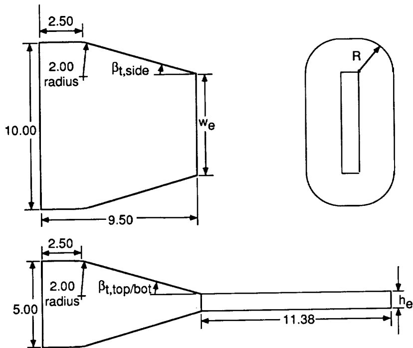
Figure 3. Geometry of nozzle with solid plume simulator. Linear dimensions are given in inches.
