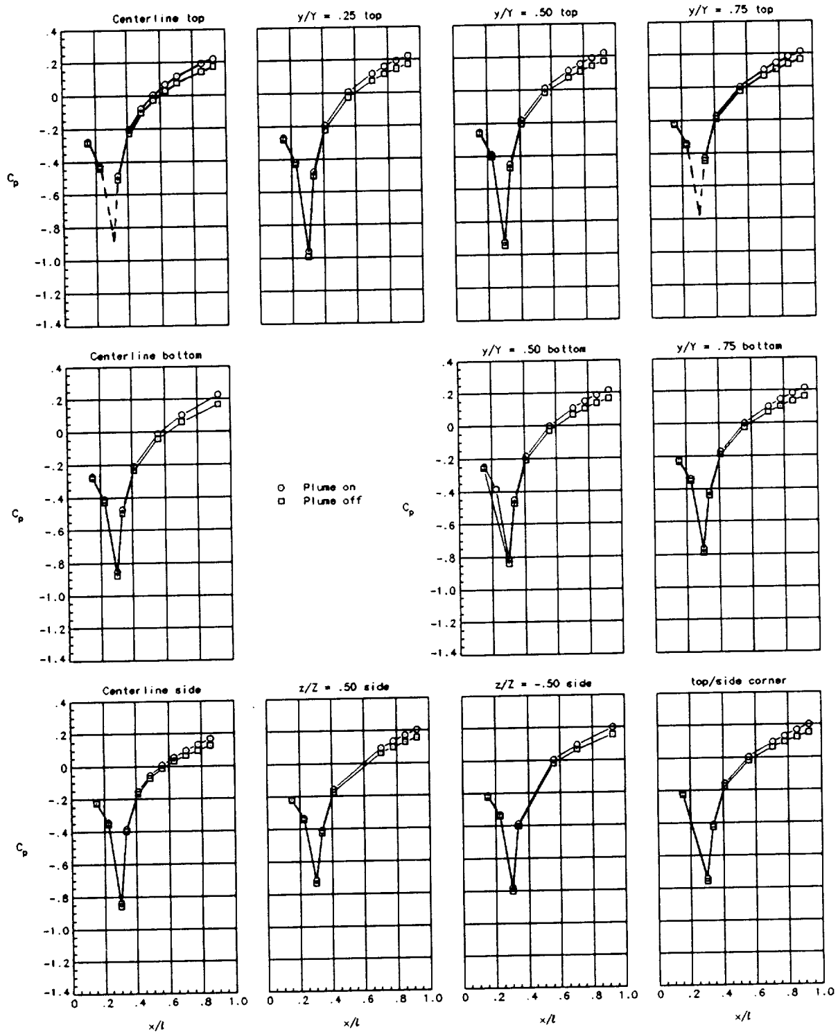
(x) Nozzle 11 with \beta_{t,top/bot} = 16.4^\circ / \beta_{t,side} = 16.4^\circ and 2-in. corner radius at M_\infty = 0.6 . C_{p,crit} = -1.290 .
