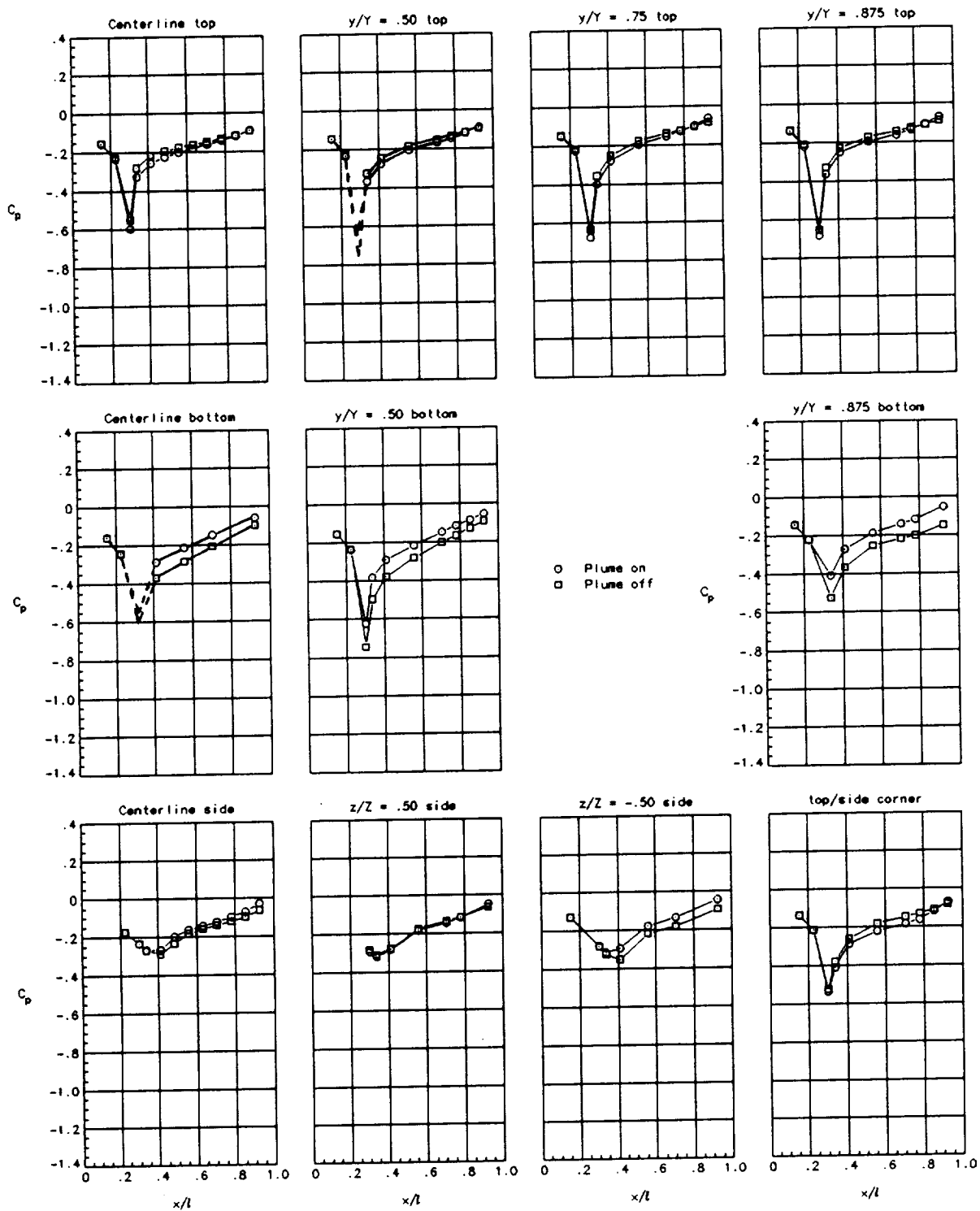
(h) Nozzle 5 with \beta_{t,top/bot} = 17.9^\circ / \beta_{t,side} = 0^\circ and 1-in. corner radius at M_\infty = 0.9 . C_{p,crit} = -0.188 .
