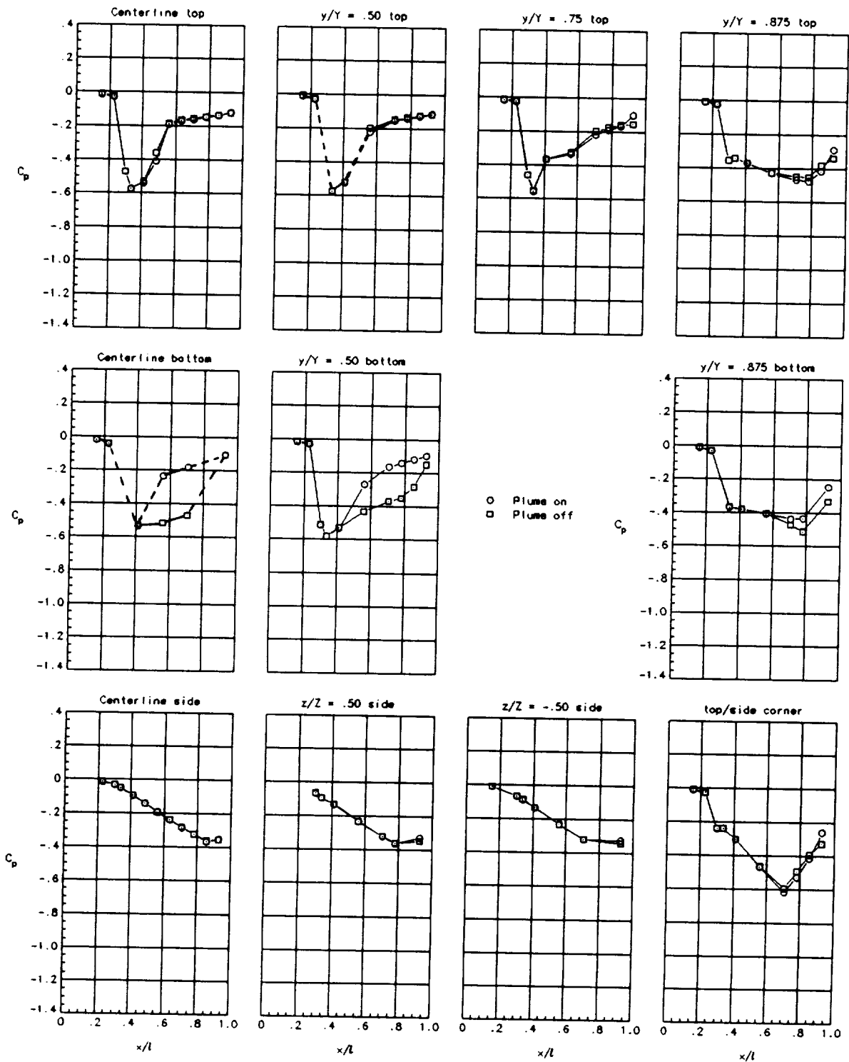
(i) Nozzle 5 with \beta_{t,top/bot} = 17.9^\circ / \beta_{t,side} = 0^\circ and 1-in. corner radius at M_\infty = 1.2 . C_{p,crit} = 0.279 .
