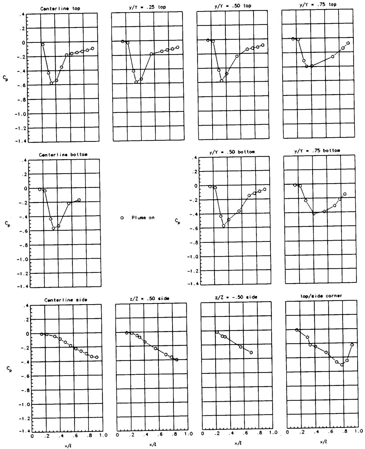
(t) Nozzle 9 with \beta_{t,top/bot} = 17.9^\circ / \beta_{t,side} = 0^\circ and 2-in. corner radius at M_\infty = 1.2 . C_{p,crit} = 0.279 .
