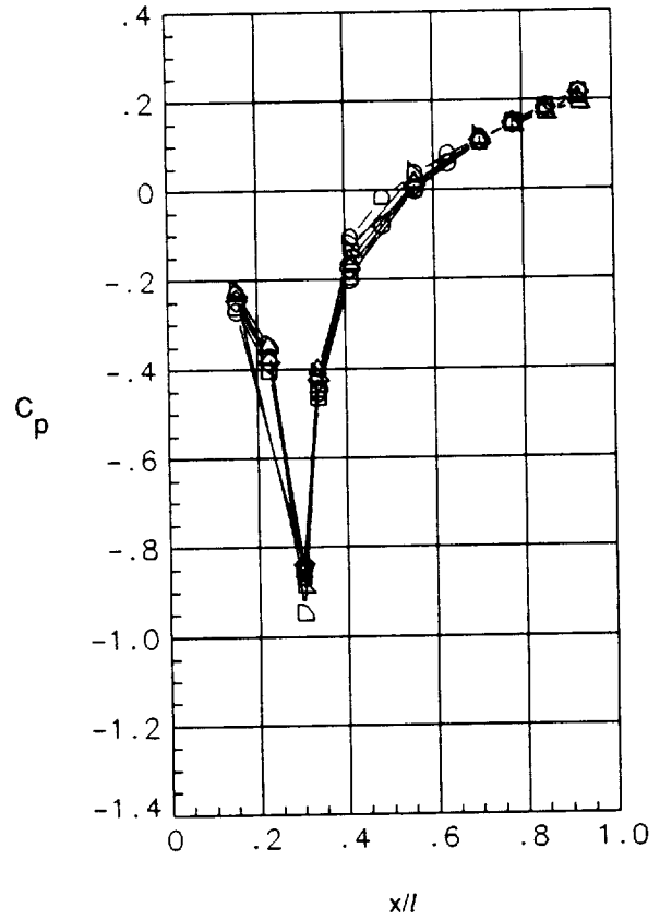
Nozzle 12: 2-in. corner radius
