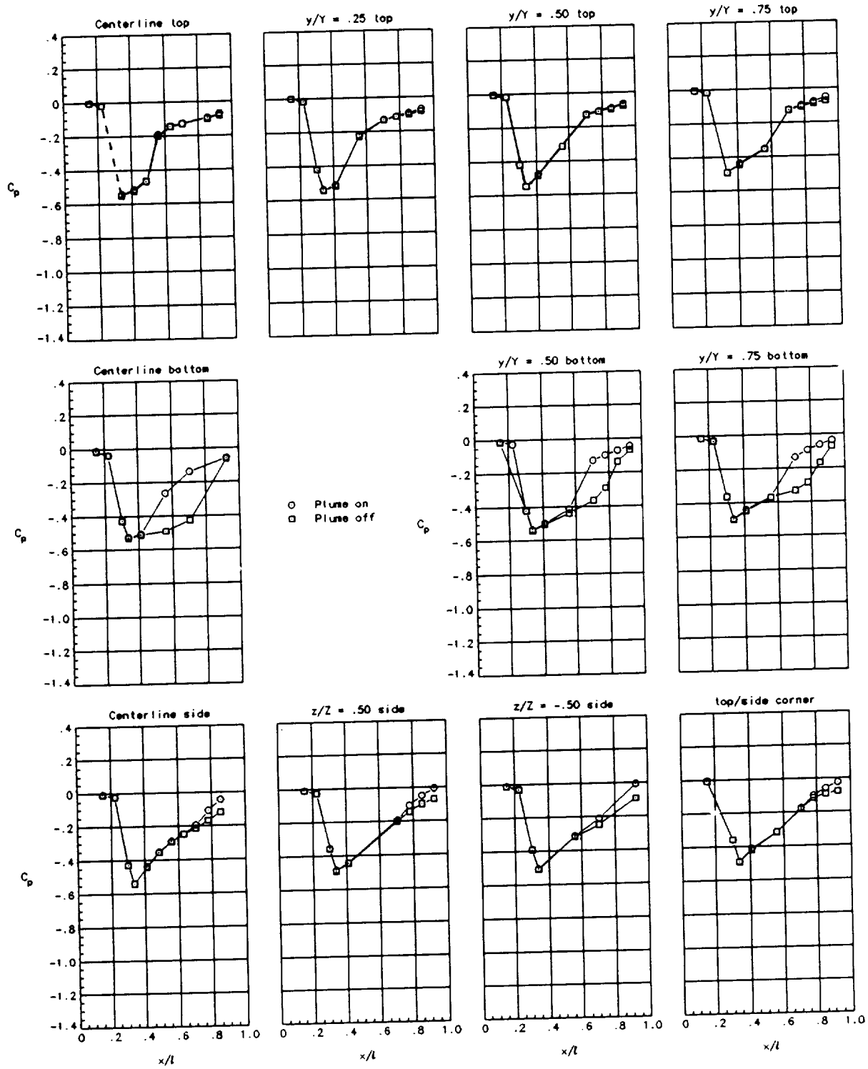
(z) Nozzle 11 with \beta_{t,top/bot} = 16.4^\circ / \beta_{t,side} = 16.4^\circ and 2-in. corner radius at M_\infty = 1.2 . C_{p,crit} = 0.279 .
