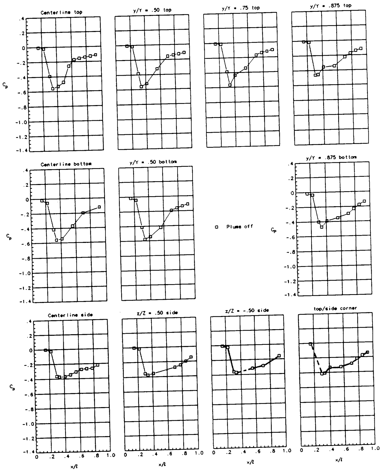
(1) Nozzle 6 with \beta_{t,top/bot} = 17.3^\circ / \beta_{t,side} = 9.7^\circ and 1-in. corner radius at M_\infty = 1.2 . C_{p,crit} = 0.279 .
