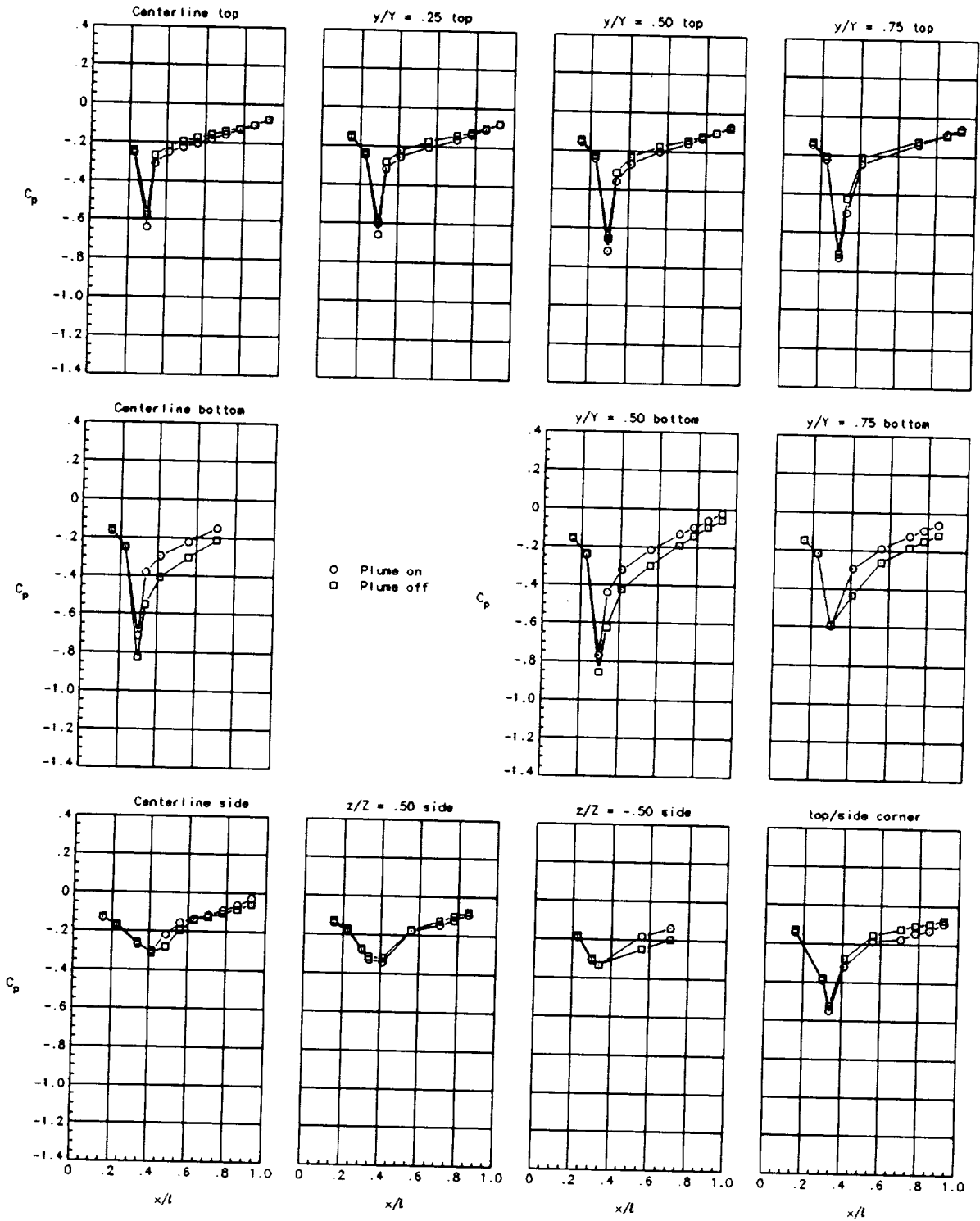
(s) Nozzle 9 with \beta_{t,top/bot} = 17.9^\circ / \beta_{t,side} = 0^\circ and 2-in. corner radius at M_\infty = 0.9 . C_{p,crit} = -0.188 .
