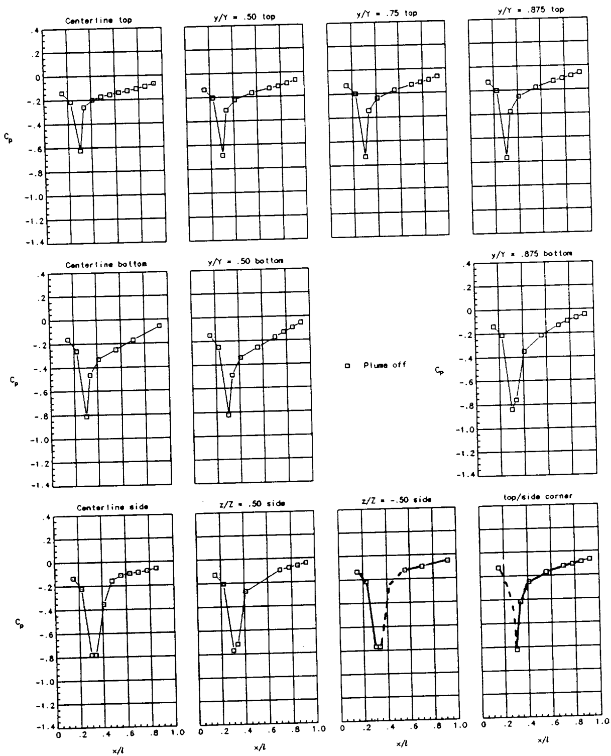
(j) Nozzle 6 with \beta_{t,top/bot} = 17.3^\circ / \beta_{t,side} = 9.7^\circ and 1-in. corner radius at M_\infty = 0.6 . C_{p,crit} = -1.290 .
