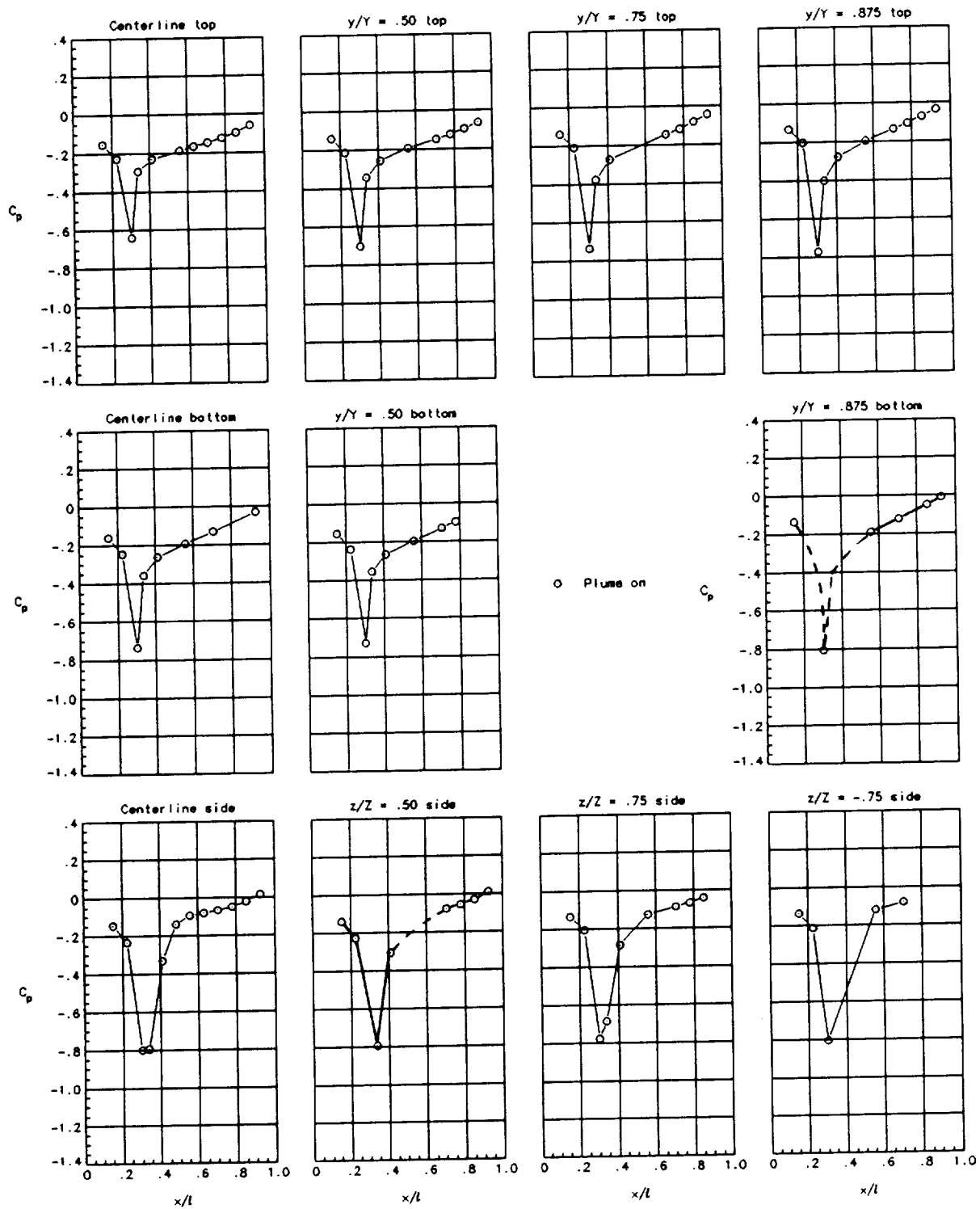
(b) Nozzle 2 with \beta_{t,top/bot} = 17.3^\circ / \beta_{t,side} = 9.7^\circ and sharp corner at M_\infty = 0.9 . C_{p,crit} = -0.188 .
