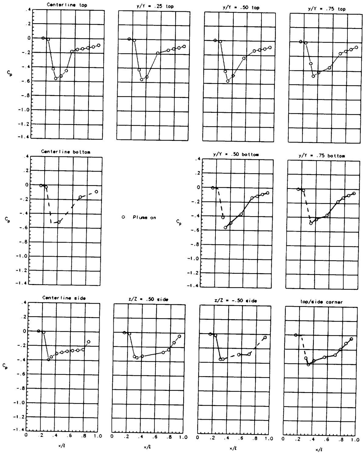
(w) Nozzle 10 with \beta_{t,top/bot} = 17.3^\circ / \beta_{t,side} = 9.7^\circ and 2-in. corner radius at M_\infty = 1.2 . C_{p,crit} = 0.279 .
