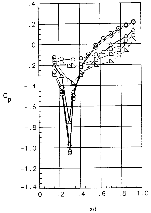
Nozzle 9: 2-in. corner radius
