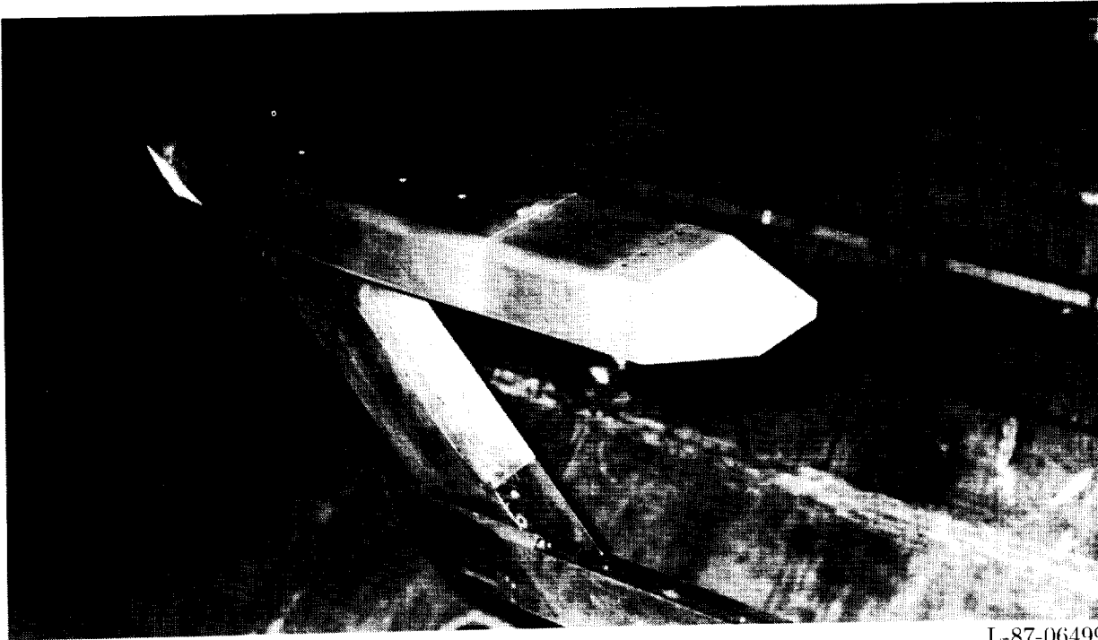
(a) Nozzle 7 without solid plume simulator.
