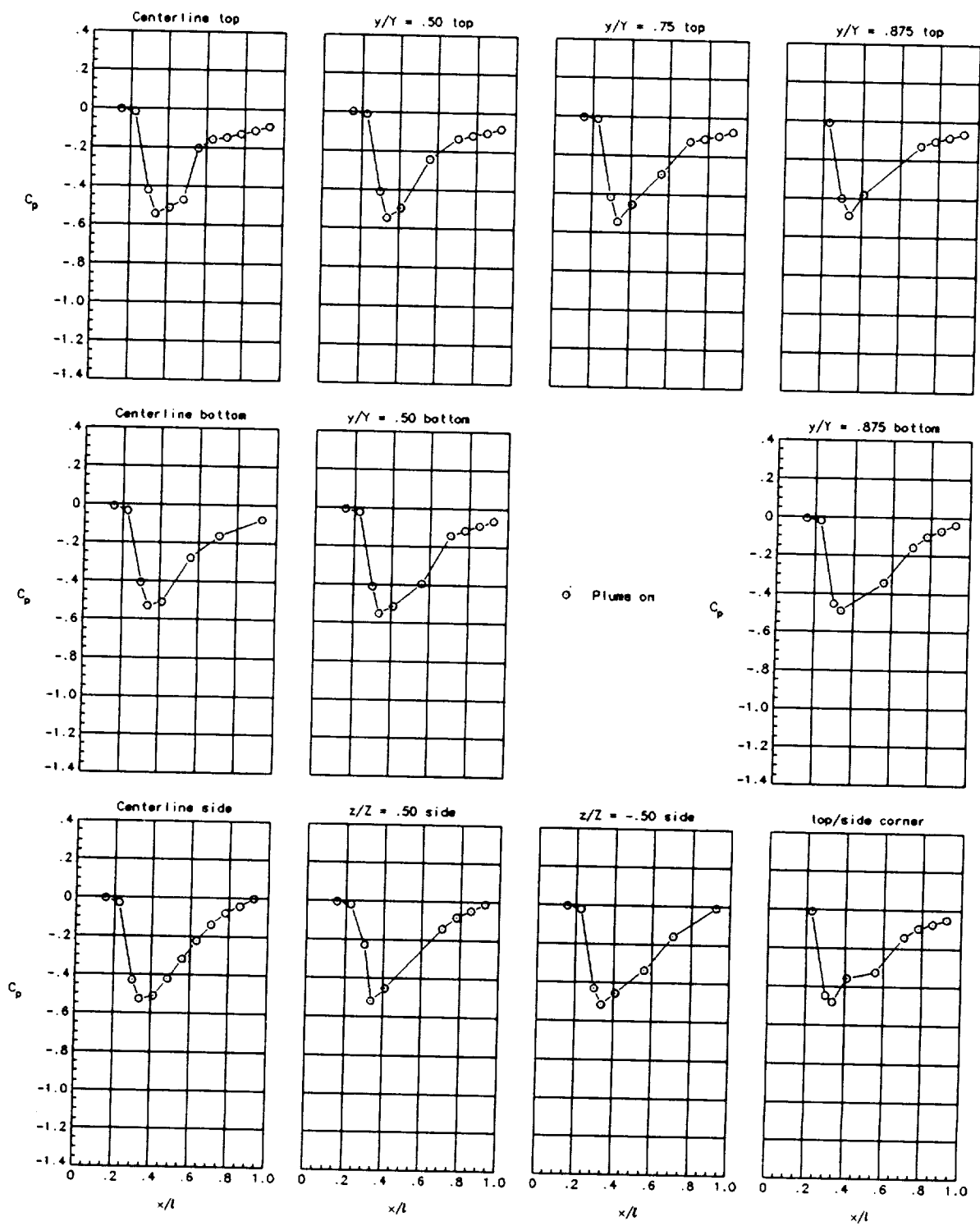
(o) Nozzle 7 with \beta_{t,top/bot} = 16.4^\circ / \beta_{t,side} = 16.4^\circ and 1-in. corner radius at M_\infty = 1.2 . C_{p,crit} = 0.279 .
