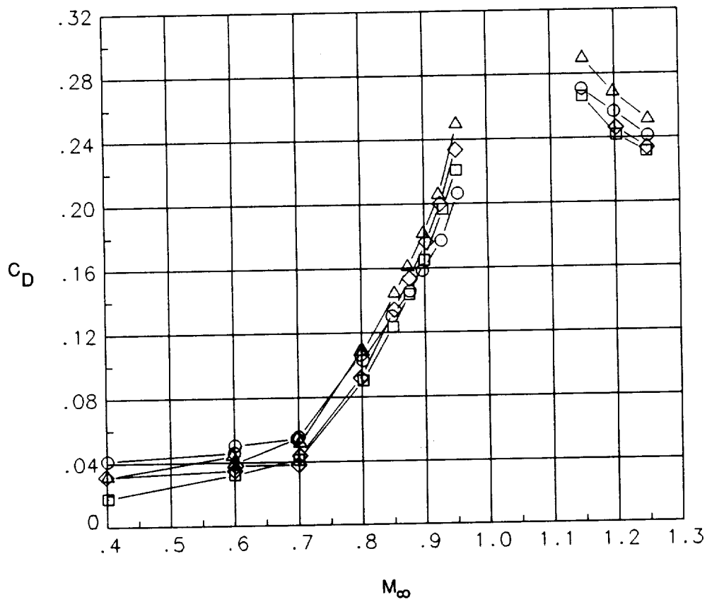
(a) Afterbody drag with plume on.
