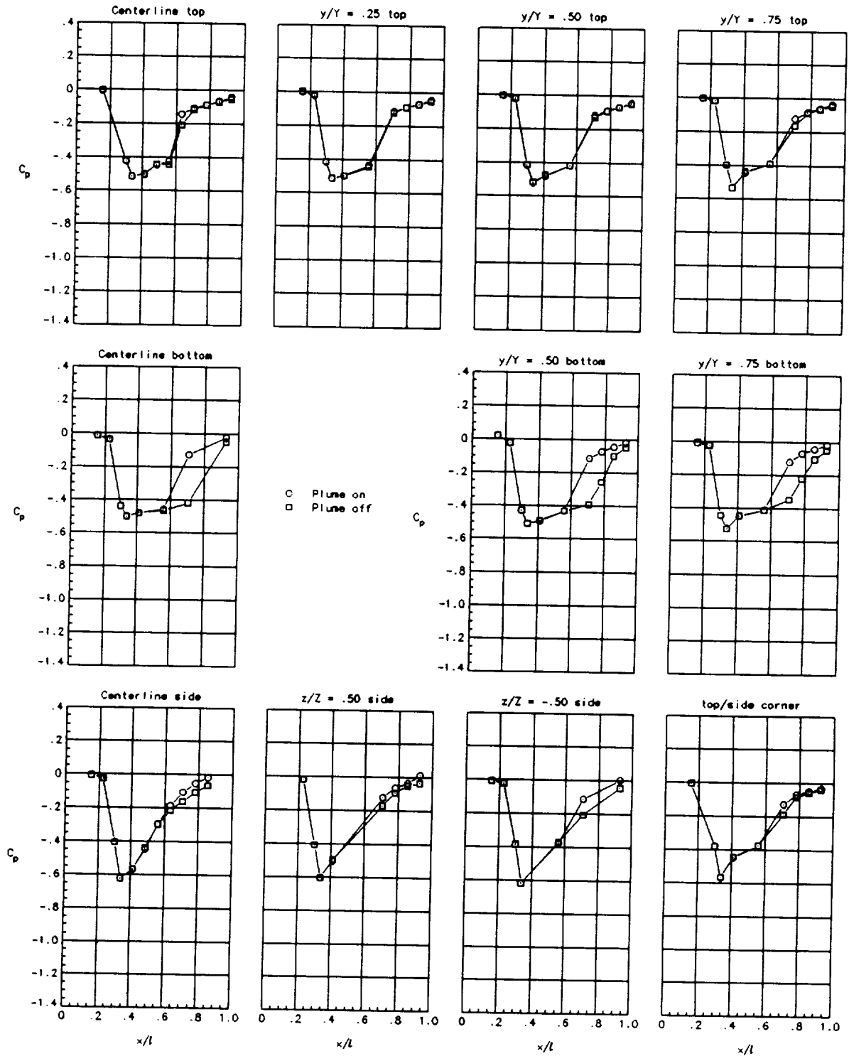
(cc) Nozzle 12 with \beta_{t,top/bot} = 15.0^\circ / \beta_{t,side} = 22.4^\circ and 2-in. corner radius at M_\infty = 1.2 . C_{p,crit} = 0.279 .
