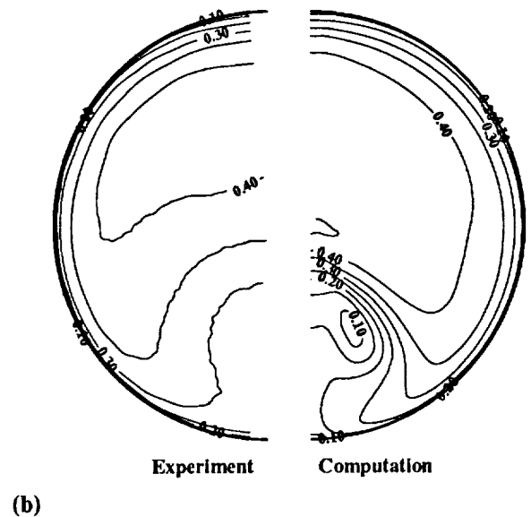
Fig. 10 Axial Mach number contours at s/D_1 = 5.73 (a) k - \epsilon turbulence model, (b) algebraic turbulence model.
