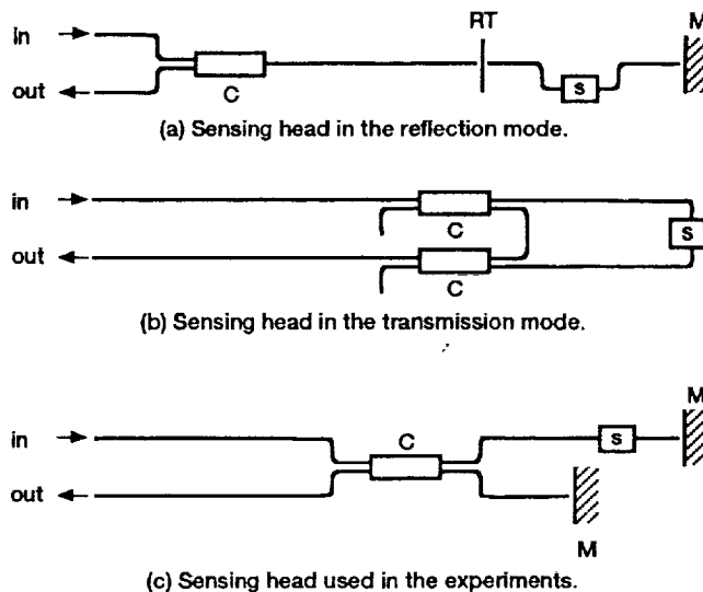
Figure 2.—Fiber optic systems.
