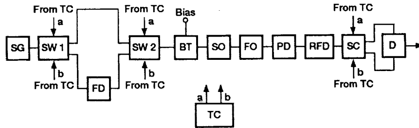
Figure 4.—Scheme using burst modulation and sequential detection.
