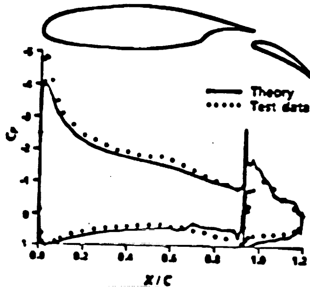
Pressure distribution - GAW-130 airfoil, flap angle 20^\circ , M = 0.3 , Re = 2.2 \times 10^6 .
