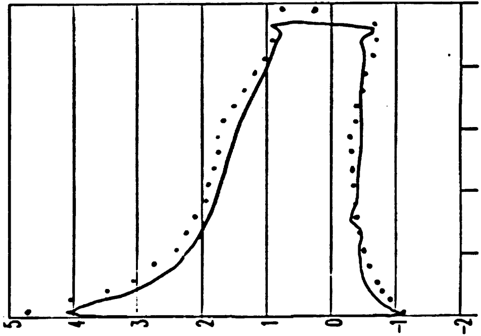
Pressure Coefficient on GA(W)-1 Airfoil, Flap Angle = 20 Degree, Re = 2.2 Million
