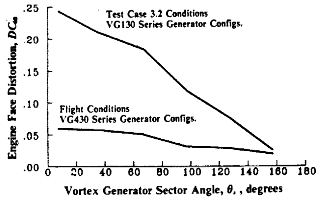
Fig. (16) - Effect of vortex generator sector angle ( \theta ), on engine face DC_{\omega} distortion, VG130 and VG430 series vortex Test Case 3.2 and flight conditions.
