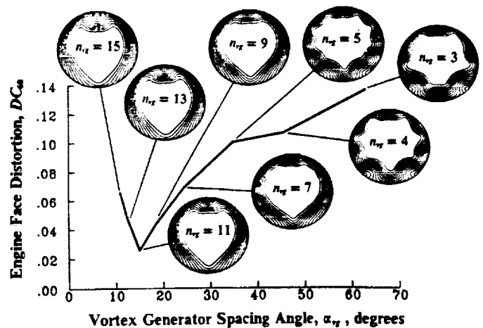
Fig. (17) - Effect of vortex generator spacing angle ( \alpha_{vg} ) on engine face DC_{\omega} distortion, VG130 series vortex generators, Test Case 3.2 initial conditions.
