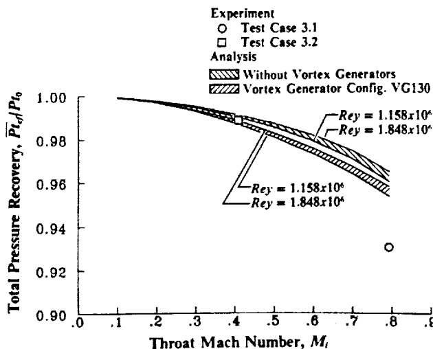
Fig. (5) - Effect of vortex flow control on engine face total pressure recovery for the RAE2129 intake duct, vortex generator configuration VG130.
