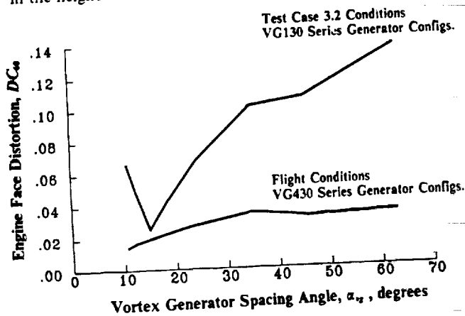
Fig. (18) - Effect of vortex generator spacing angle ( \alpha_{vg} ) on engine face DC_{\omega} distortion, VG130 and VG430 series vortex generators, Test Case 3.2 and flight conditions.
