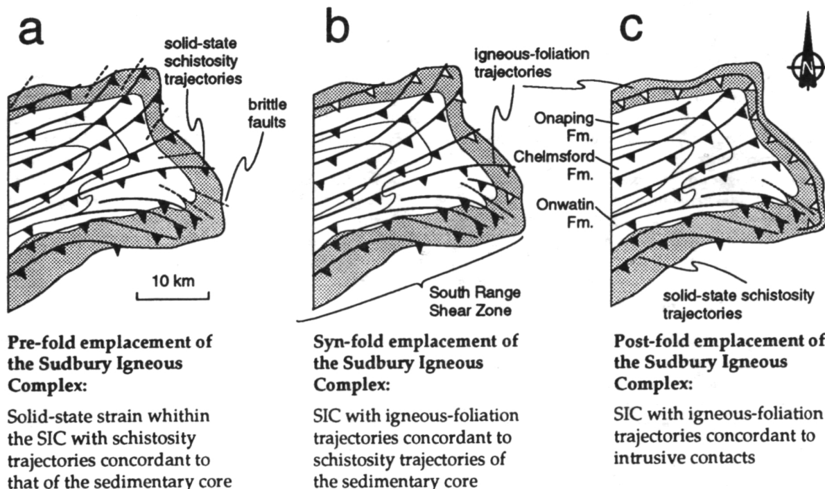
Fig. 1. Eastern Sudbury structure: SIC (shaded), Whitewater Group (white).
